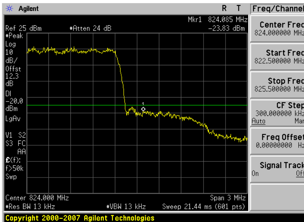
Plot 7-8. Exterior Band Edge Plot (BC10 CDMA Ch. 684) - $90.691
