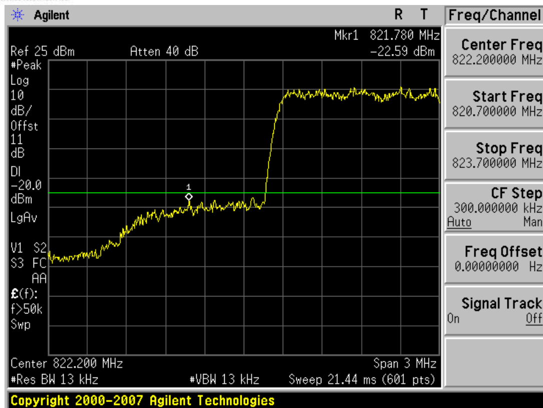
Plot 7-9. Interior Band Edge Plot (BC10 CDMA Ch. 684) - $90.691
