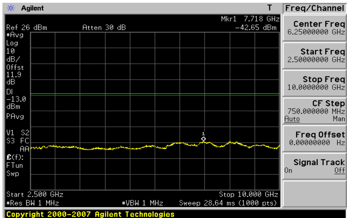
Plot 7-2. Conducted Spurious Plot (BC10 CDMA Ch. 476)
