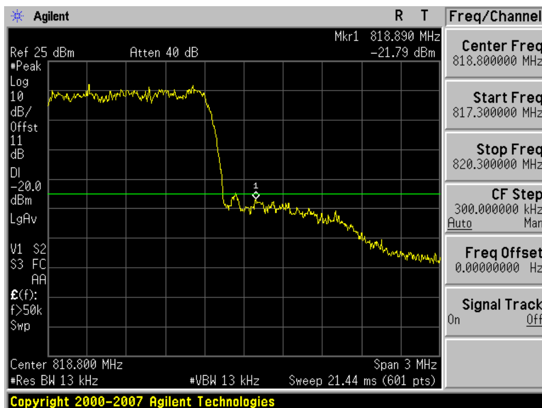
Plot 7-4. Interior Band Edge Plot (BC10 CDMA Ch. 476) - $90.691
