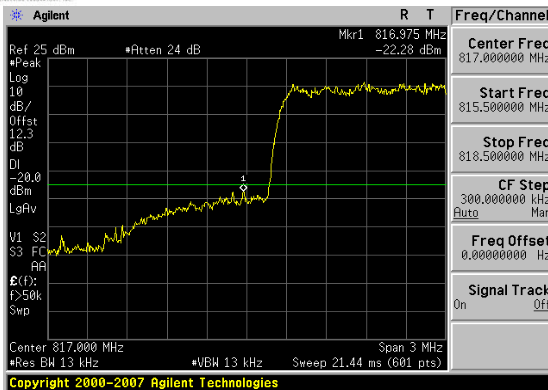
Plot 7-3. Exterior Band Edge Plot (BC10 CDMA Ch. 476) - $90.691
