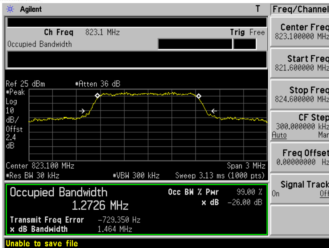
Plot 7-5. Occupied Bandwidth Plot (BC10 CDMA Ch. 684)
