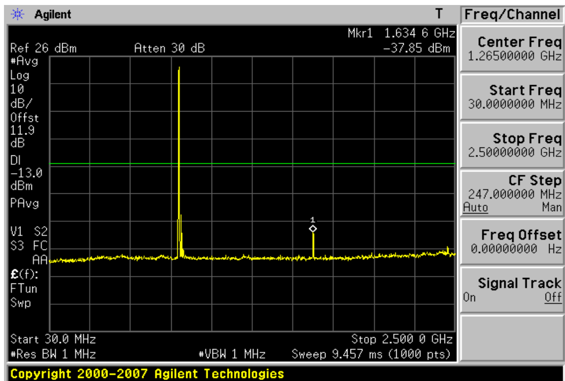
Plot 7-1. Conducted Spurious Plot (BC10 CDMA Ch. 476)
