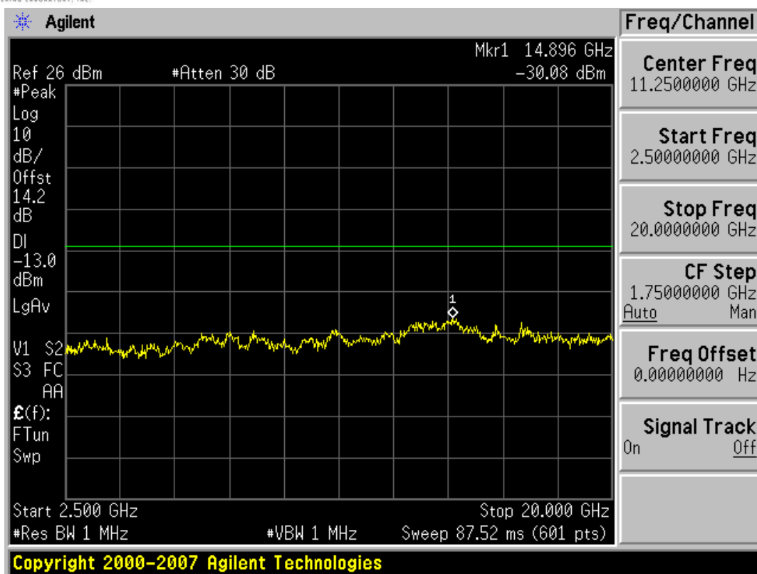
Plot 7-25. Conducted Spurious Plot (PCS CDMA Mode – Ch. 1275)
