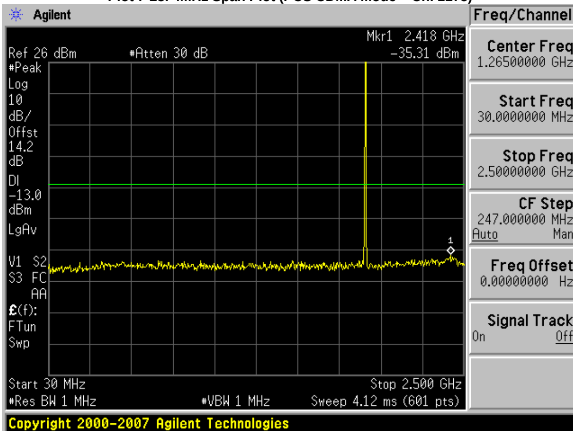
Plot 7-24. Conducted Spurious Plot (PCS CDMA Mode - Ch. 1275)
