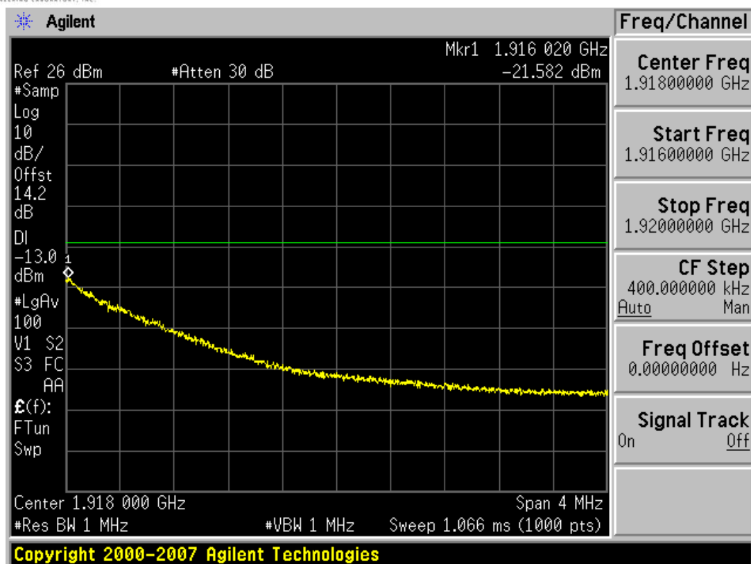
Plot 7-27. 4MHz Span Plot (PCS CDMA Mode – Ch. 1275)
