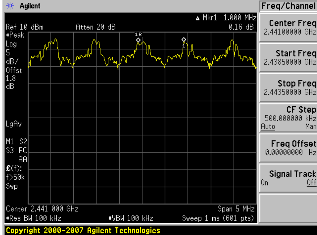
Plot 6-14. Channel Spacing Plot (Bluetooth)
