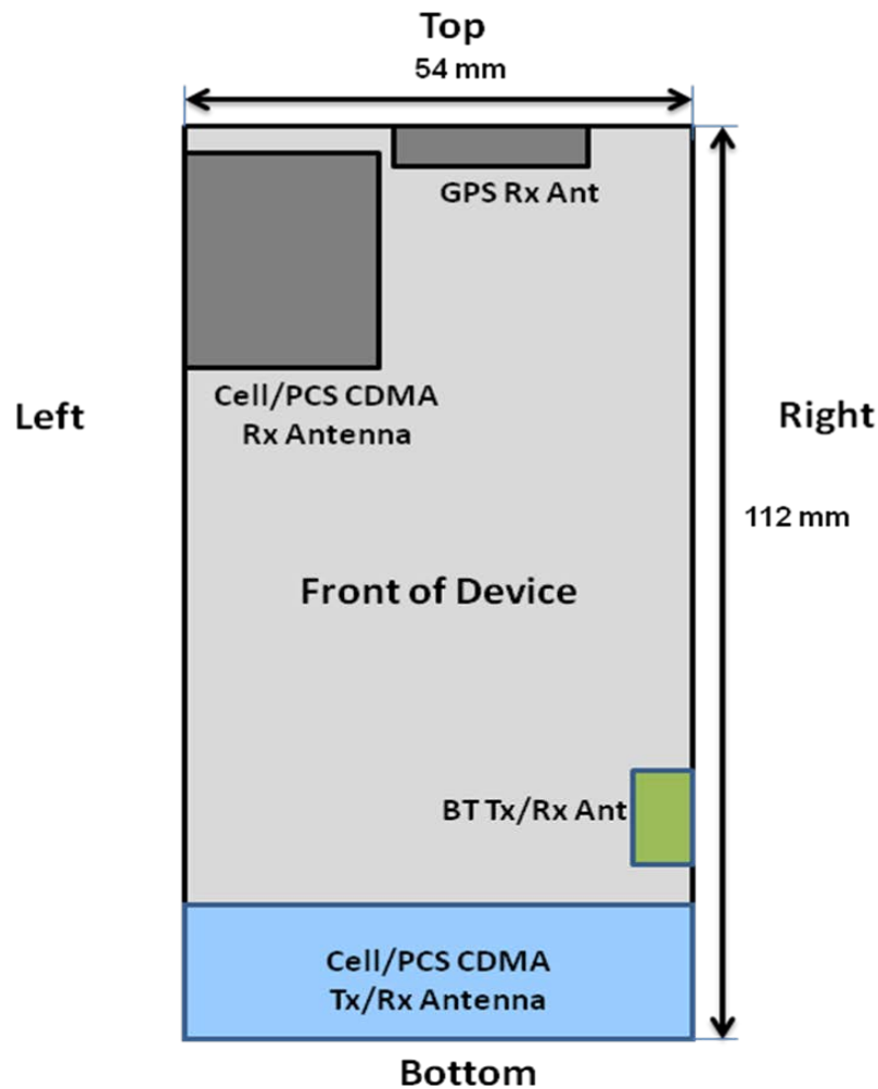
Figure 1-1 DUT Antenna Locations
