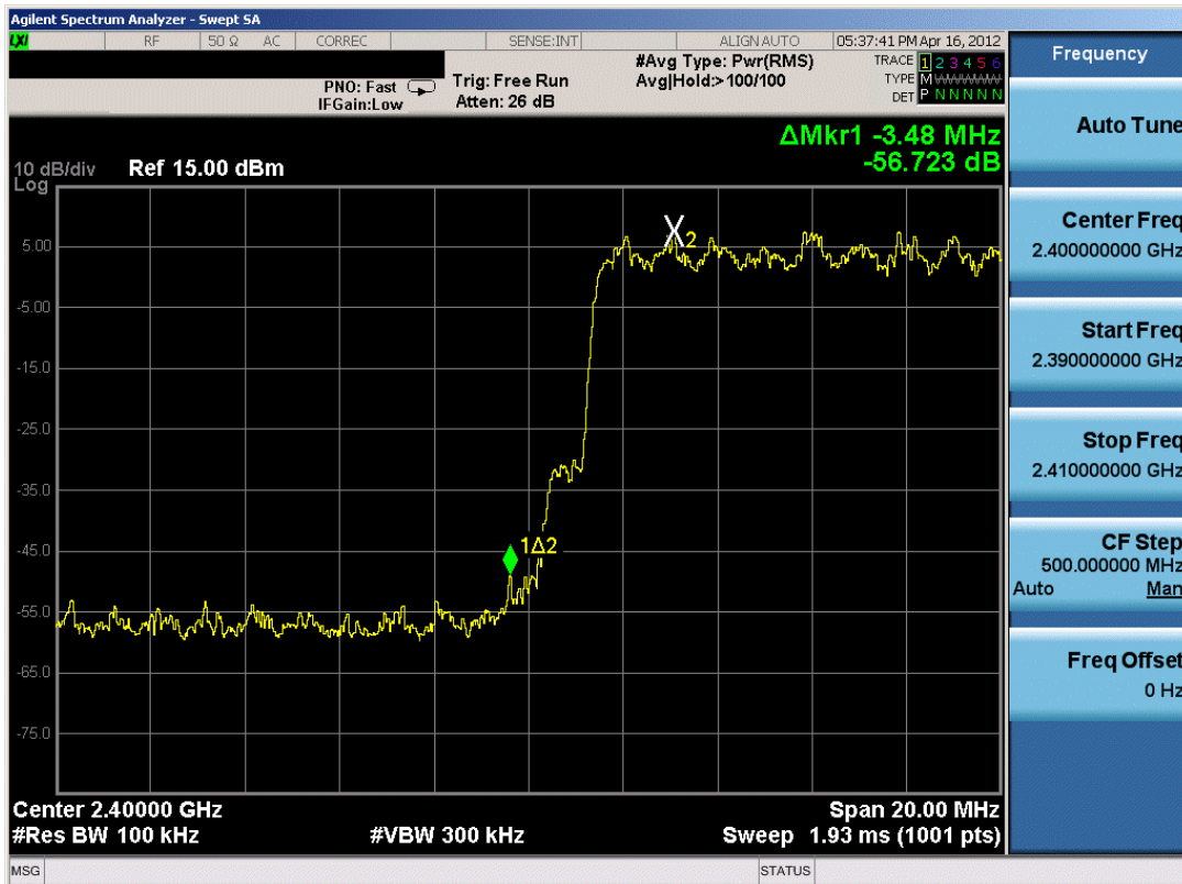
Plot 6-12. Band Edge Plot (Bluetooth with Hopping Enabled, 2Mbps)
