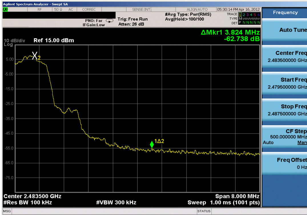
Plot 6-11. Band Edge Plot (Bluetooth with Hopping Disabled, 2Mbps – Ch. 78)
