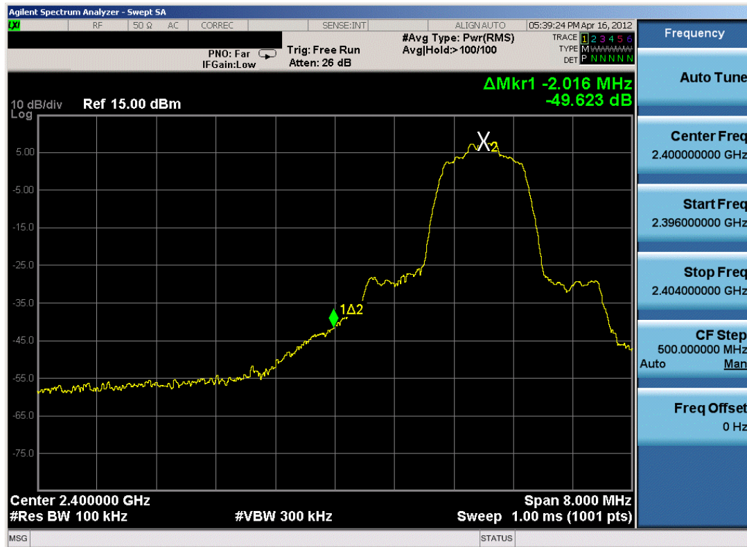
Plot 6-10. Band Edge Plot (Bluetooth with Hopping Disabled, 2Mbps – Ch. 0)
