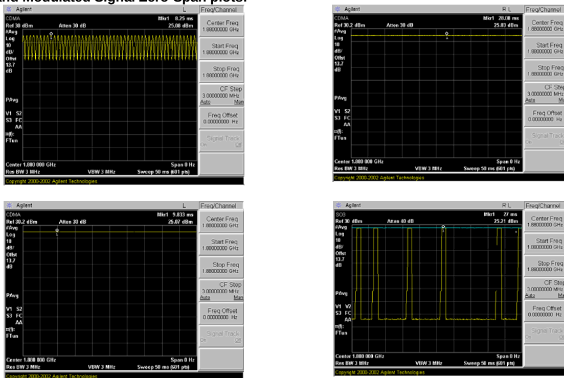
Figure 8-4 Zero-Span Plots
