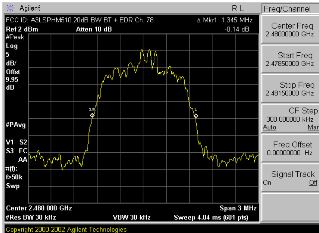
Plot 6-3. 20dB Bandwidth Plot (Bluetooth 2.0 w/ Enhanced Data Rate – Ch. 78)
