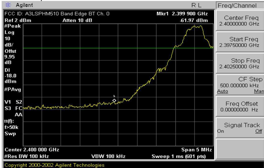
Plot 6-4. Band Edge Plot (Bluetooth 1.2 – Ch. 0)
