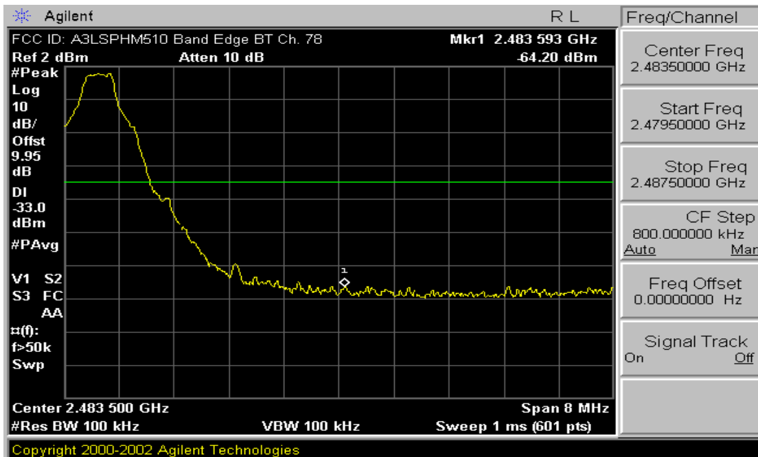
Plot 6-5. Band Edge Plot (Bluetooth 1.2 – Ch. 78)
