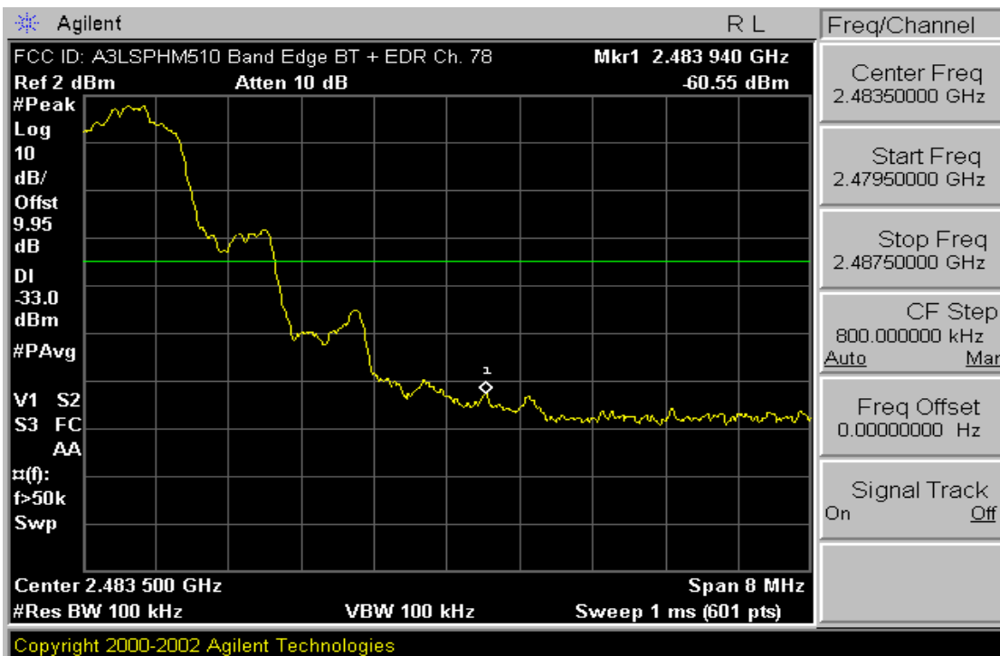
Plot 6-7. Band Edge Plot (Bluetooth 2.0 w/ Enhanced Data Rate – Ch. 78)
