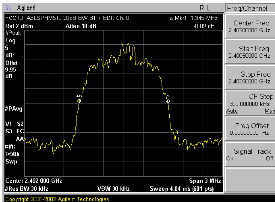
Plot 6-1. 20dB Bandwidth Plot (Bluetooth 2.0 w/ Enhanced Data Rate – Ch. 0)
