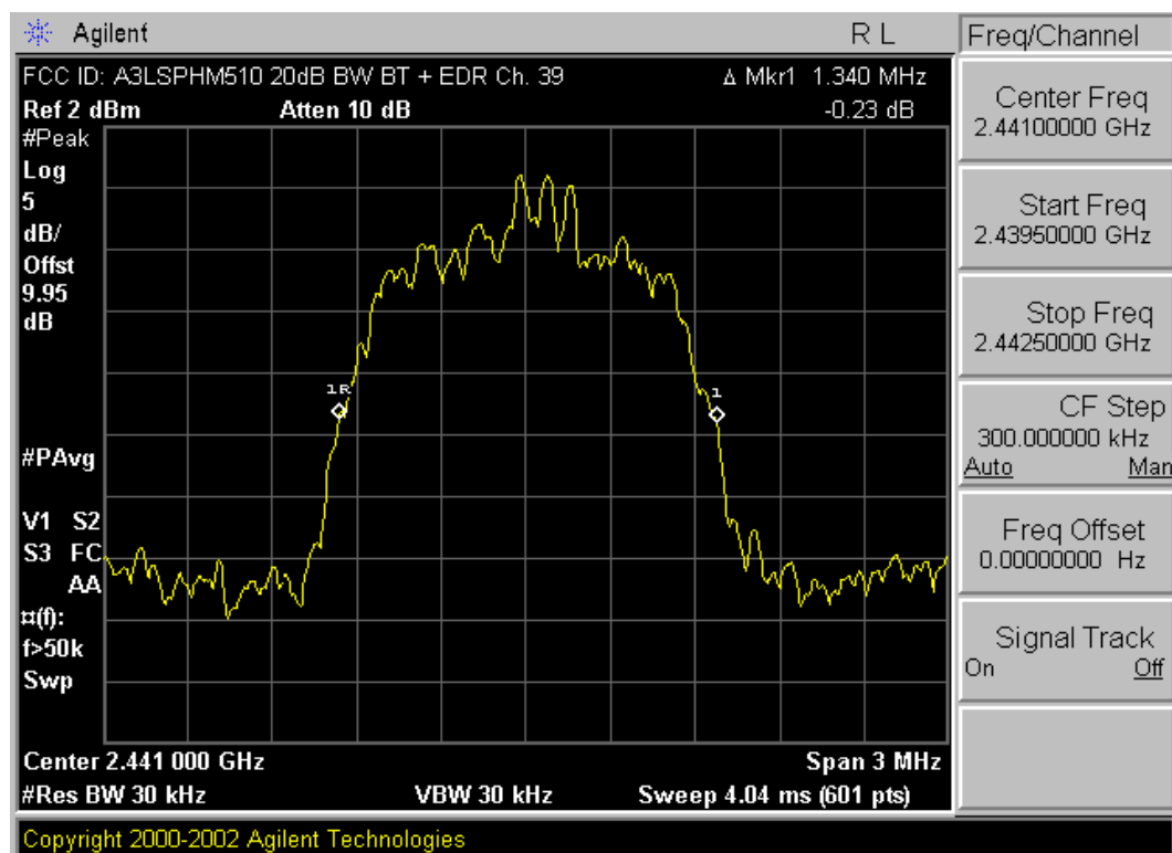
Plot 6-2. 20dB Bandwidth Plot (Bluetooth 2.0 w/ Enhanced Data Rate – Ch. 39)
