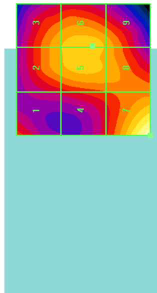
Figure 10-2 Sample H-field Scan Overlay (See Test Setup Photographs for actual WD overlay)
