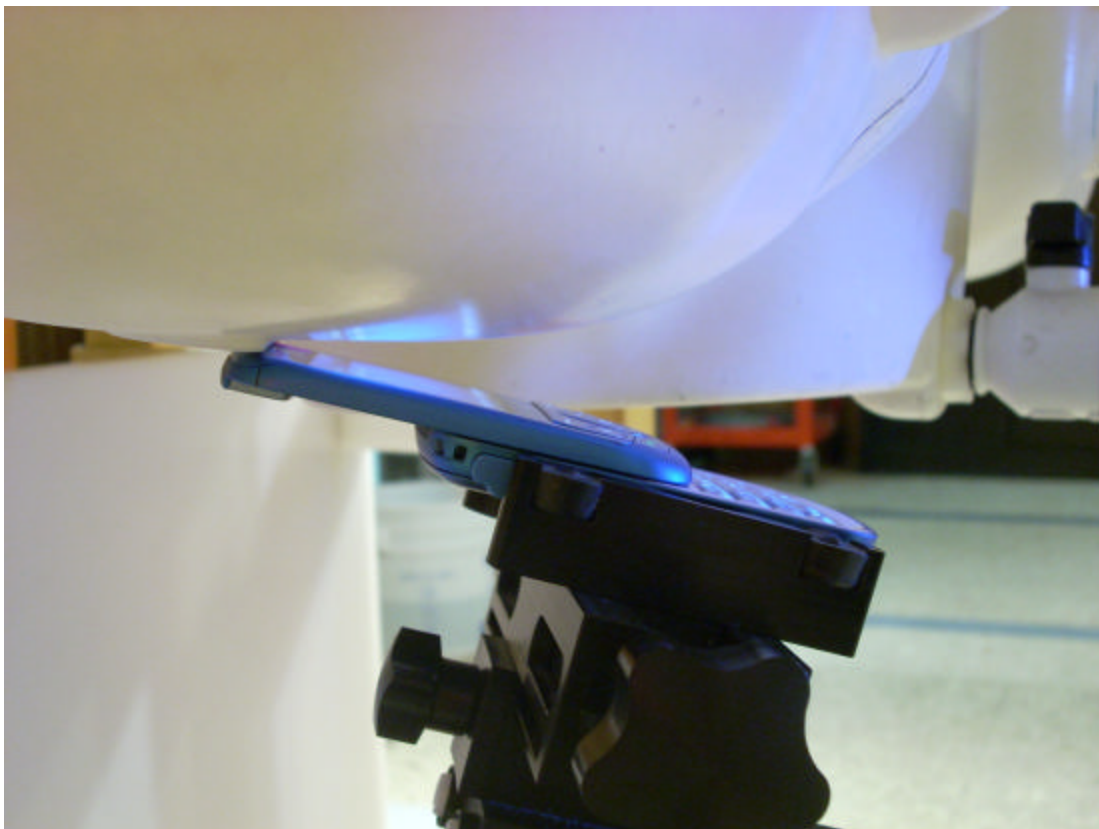
Figure 6: Right Head SAR, 15° Tilt, Slide Out
