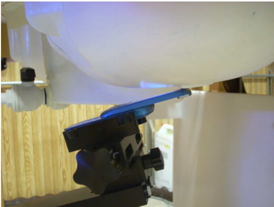
Figure 10: Left Head SAR, 15° Tilt, Slide Out
