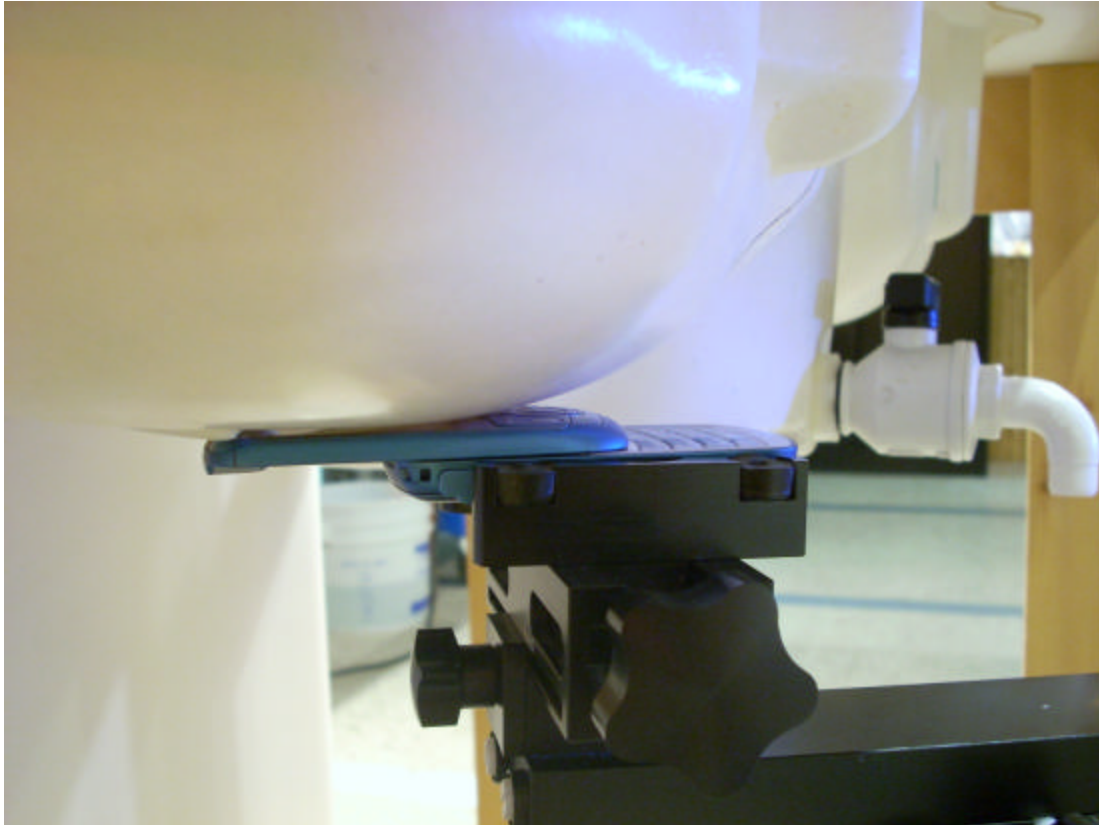
Figure 5: Right Head SAR, Cheek Touch, Slide Out
