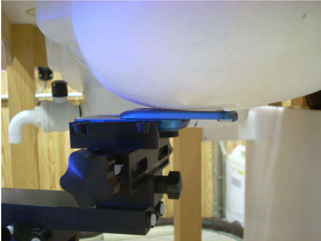
Figure 9: Left Head SAR, Cheek Touch, Slide Out
