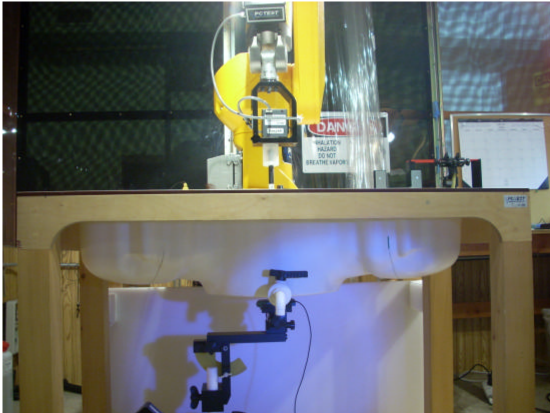
Figure 11: Body SAR
