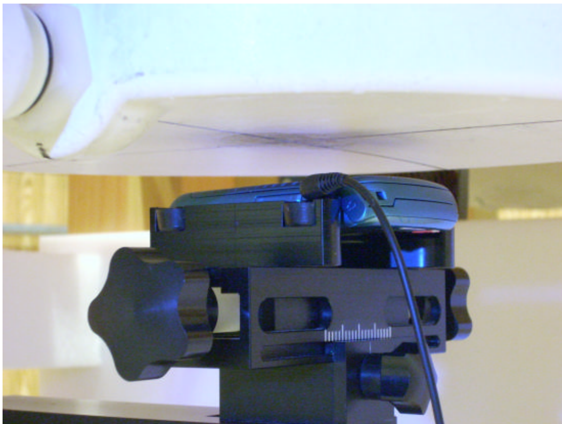
Figure 12: Body SAR, Back Side with 15mm Space
