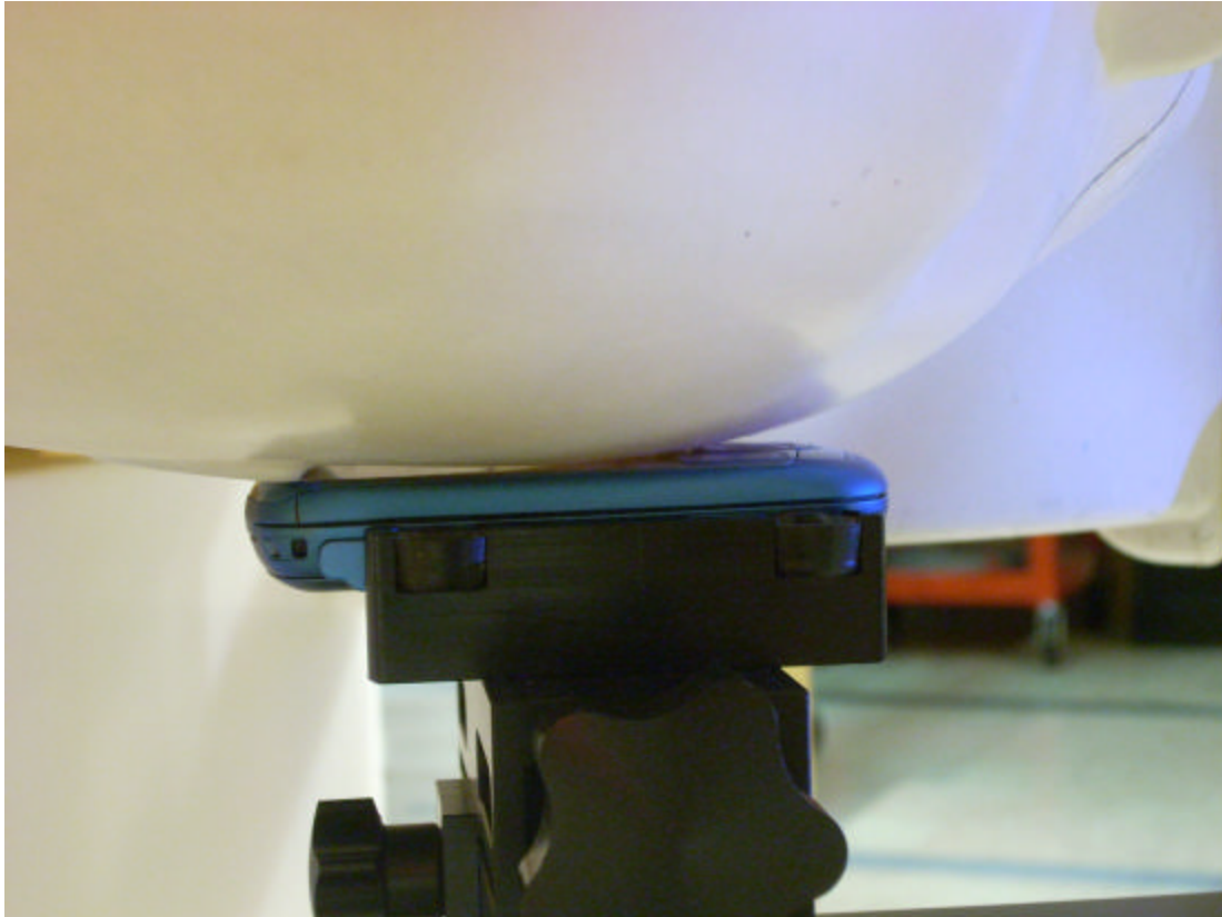
Figure 3: Right Head SAR, Cheek Touch, Slide In
