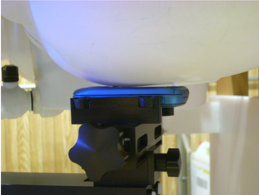
Figure 7: Left Head SAR, Cheek Touch, Slide In
