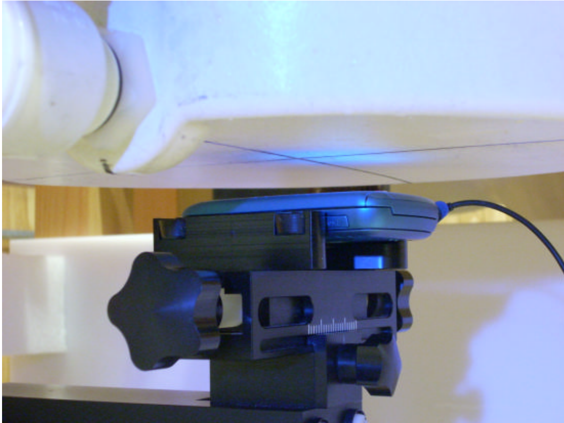
Figure 12: Body SAR, Front Side with 15mm Space
