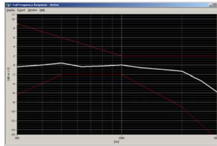
Figure 6-1 Axial Frequency Response
