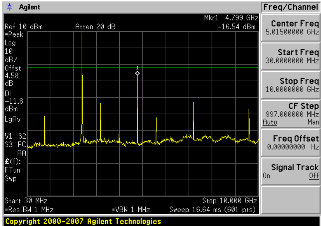
Plot 6-18. Conducted Spurious Plot (Bluetooth, 2Mbps – Ch. 0)
