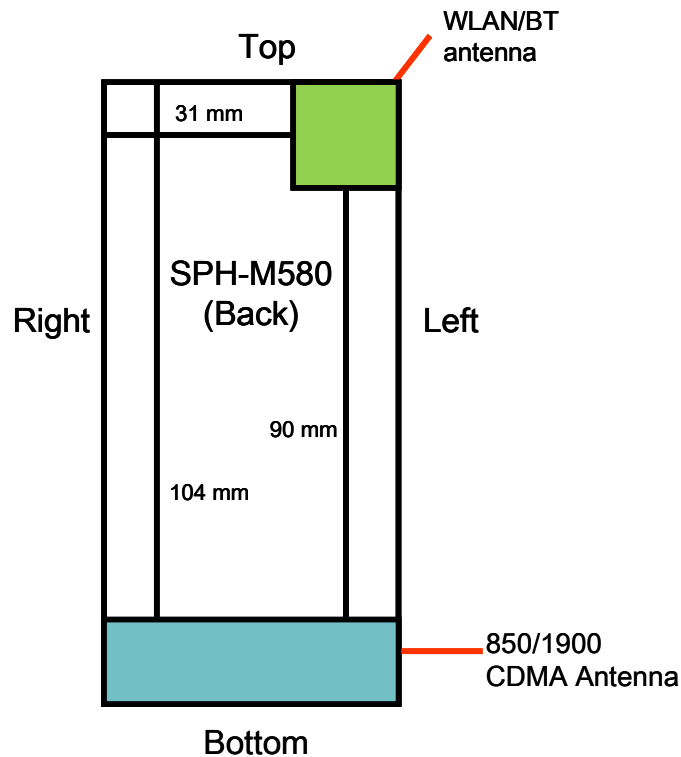
Figure 13-1 Identification of Sides for SAR Testing
