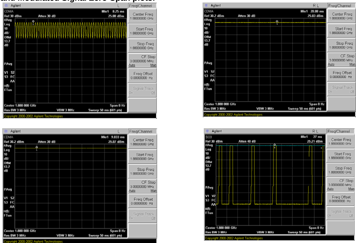
Figure 8-4 Zero-Span Plots
