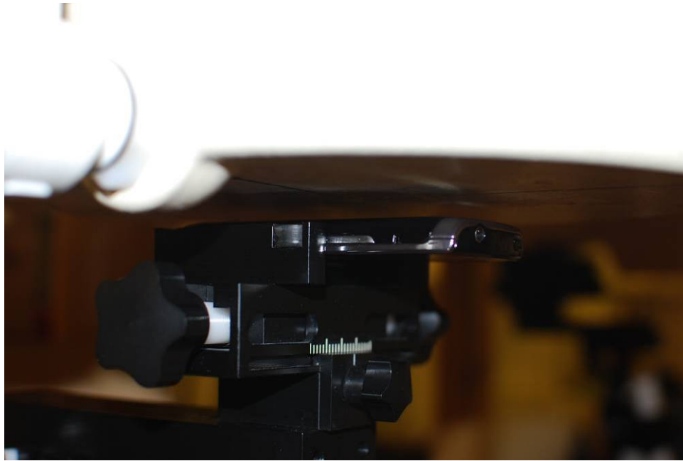
Figure 21-5 SAR Test Setup Photo 5 – Back at 1.0 cm
