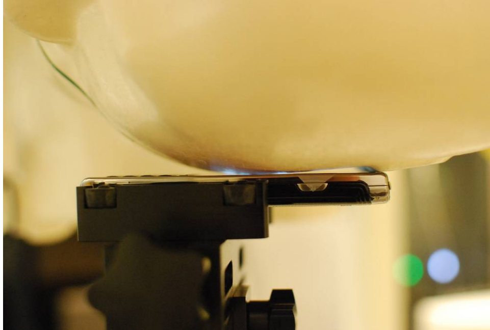
Figure 21-3 SAR Test Setup Photo 3 – Left Touch
