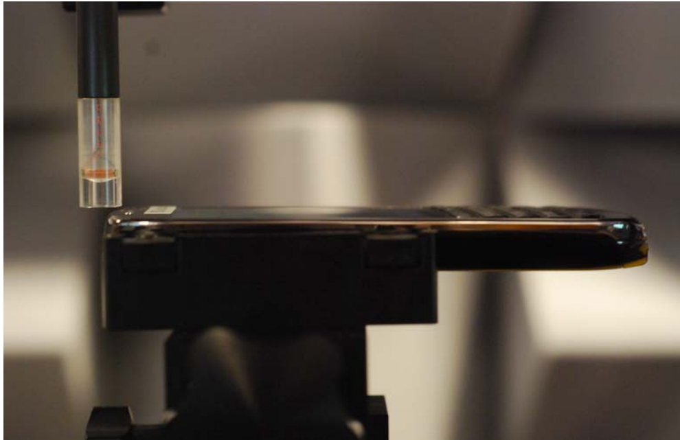
Figure 13-1 Test Setup for Wireless Device
