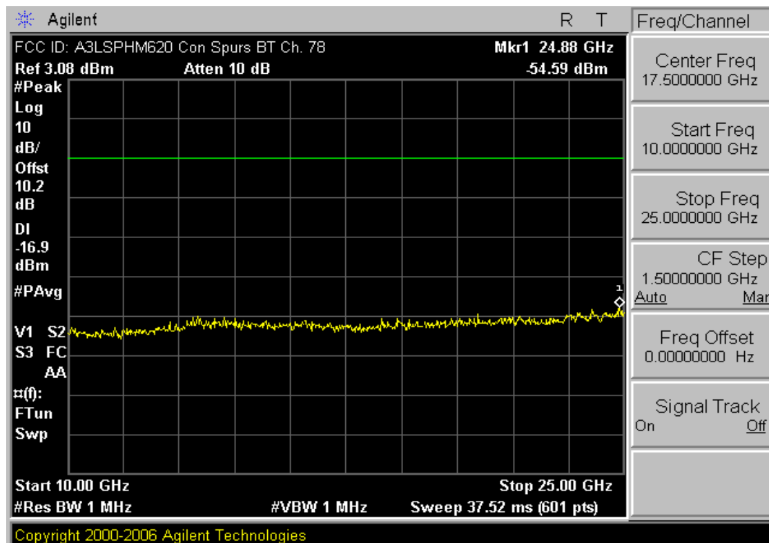
Plot 6-17. Conducted Spurious Plot (Bluetooth – Ch. 78)
