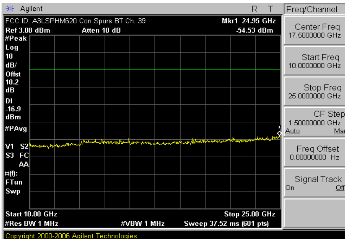
Plot 6-15. Conducted Spurious Plot (Bluetooth – Ch. 39)
