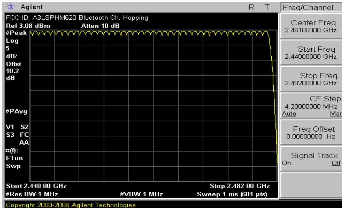
Plot 6-11. High End Spectrum Channel Hopping Plot (Bluetooth)
