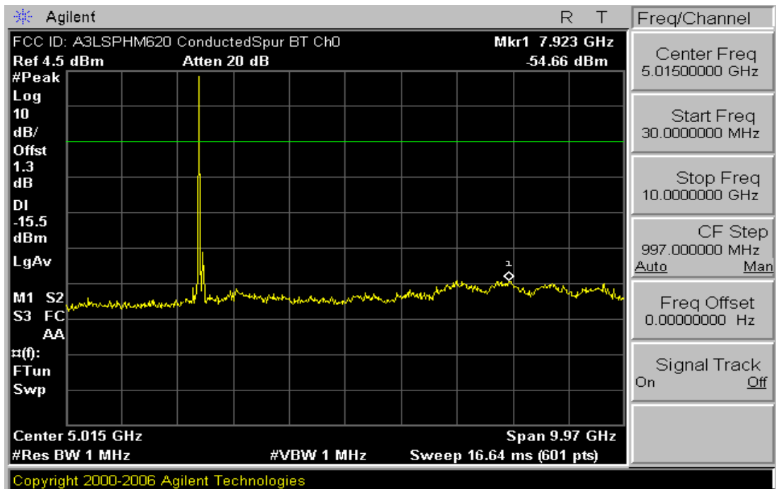
Plot 6-12. Conducted Spurious Plot (Bluetooth – Ch. 0)
