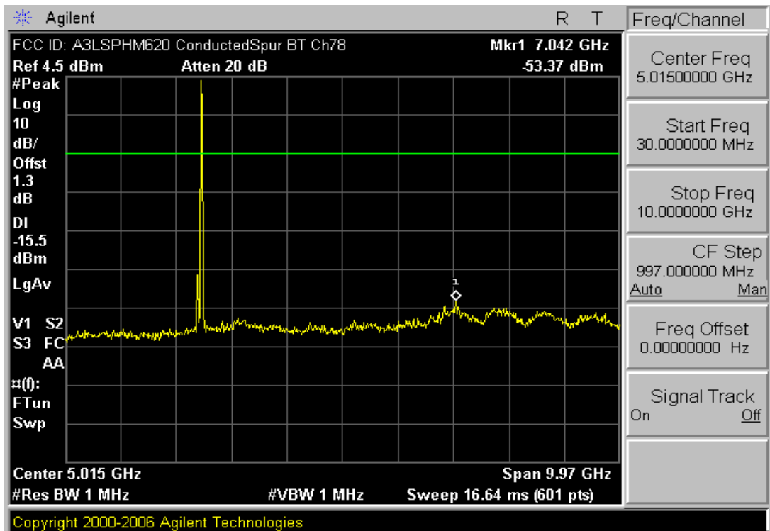
Plot 6-16. Conducted Spurious Plot (Bluetooth – Ch. 78)
