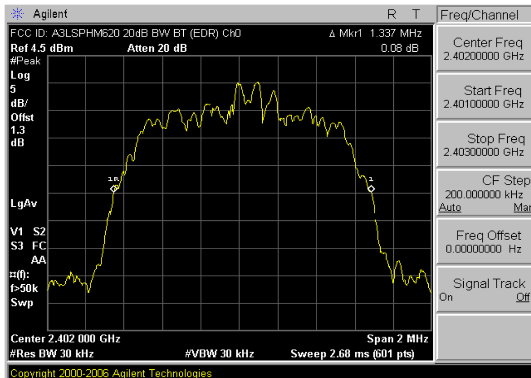
Plot 6-1. 20dB Bandwidth Plot (Bluetooth 2.0 with Enhanced Data Rate – Ch. 0)
