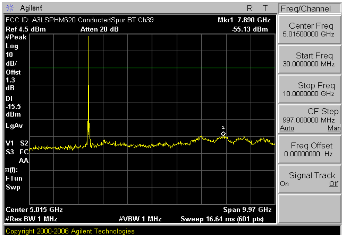
Plot 6-14. Conducted Spurious Plot (Bluetooth – Ch. 39)
