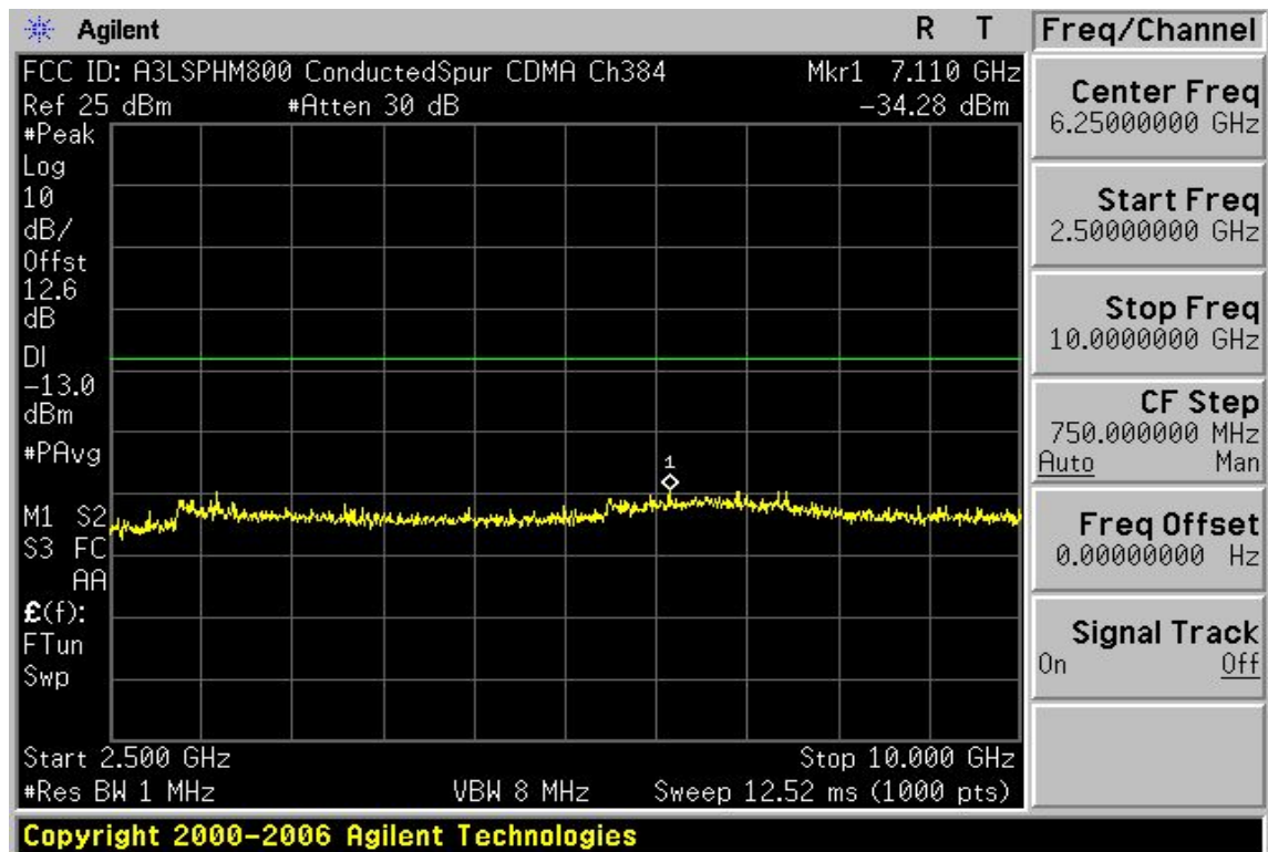
Plot 7-6. Conducted Spurious Plot (Cellular CDMA Mode – Ch. 384)
