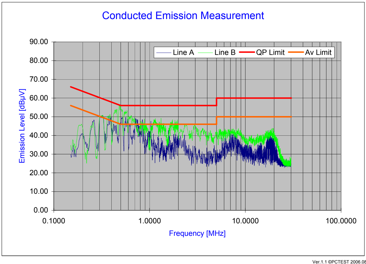
Plot 6-1. Line Conducted Plot with Bluetooth
