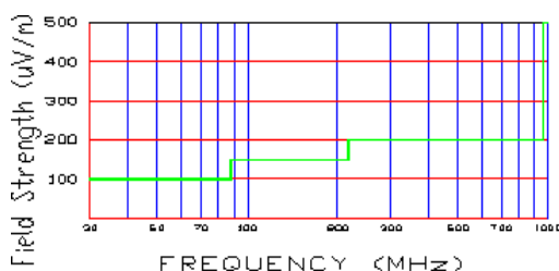
Figure 6-2. 3-Meter Limits
