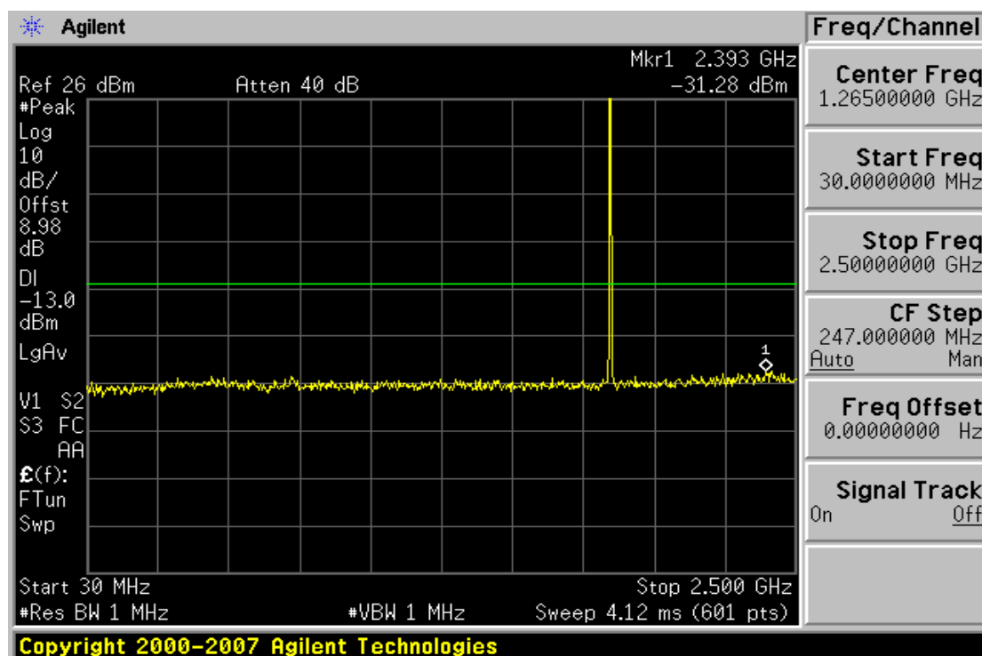
Plot 7-1. Conducted Spurious Plot (PCS CDMA Mode – Ch. 25)
