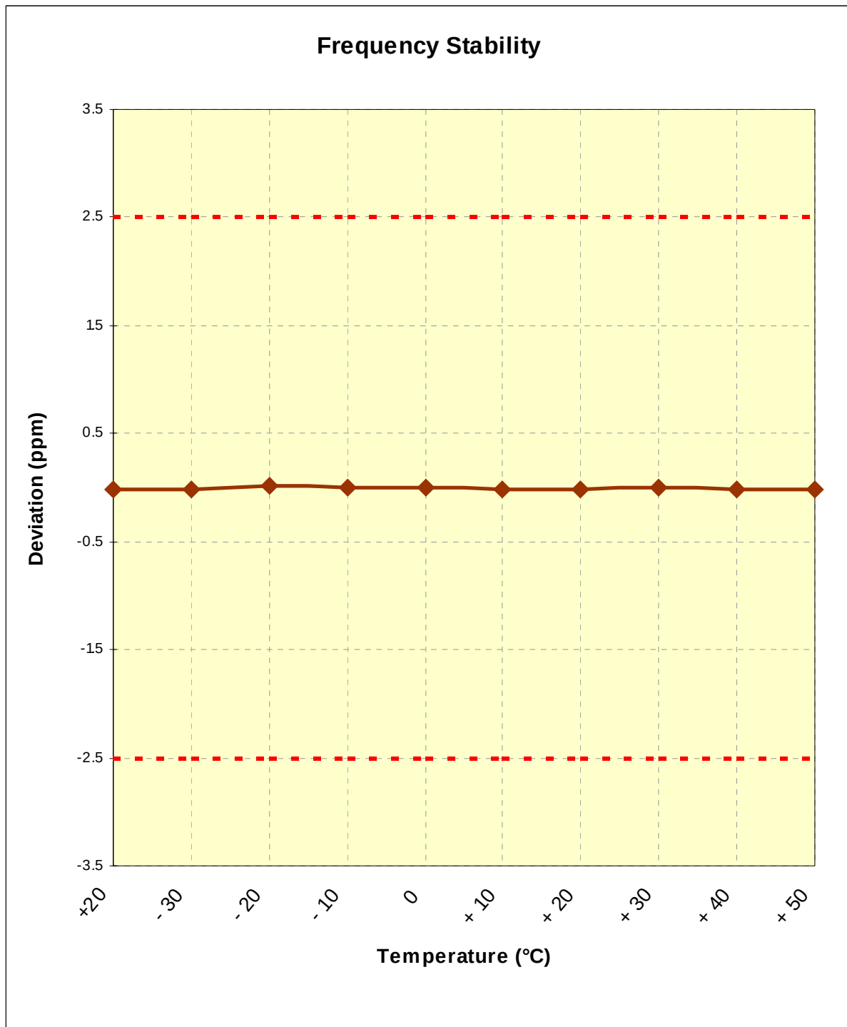
Figure 6-1. Frequency Stability Graph (PCS CDMA Mode – Ch. 600)
