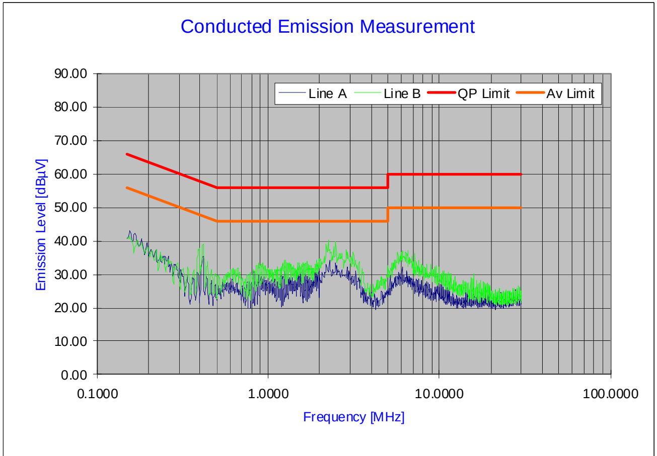
Plot 6-15. Line Conducted Plot with Bluetooth (LE)
