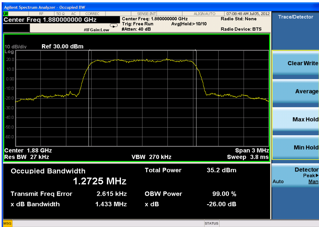
Plot 7-7. Occupied Bandwidth Plot (PCS CDMA Mode – Ch. 600)
