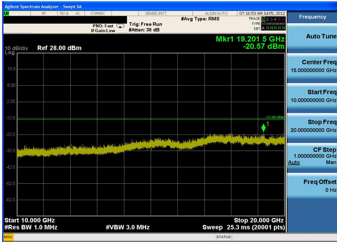
Plot 7-2. Conducted Spurious Plot (PCS CDMA Mode – Ch. 25)
