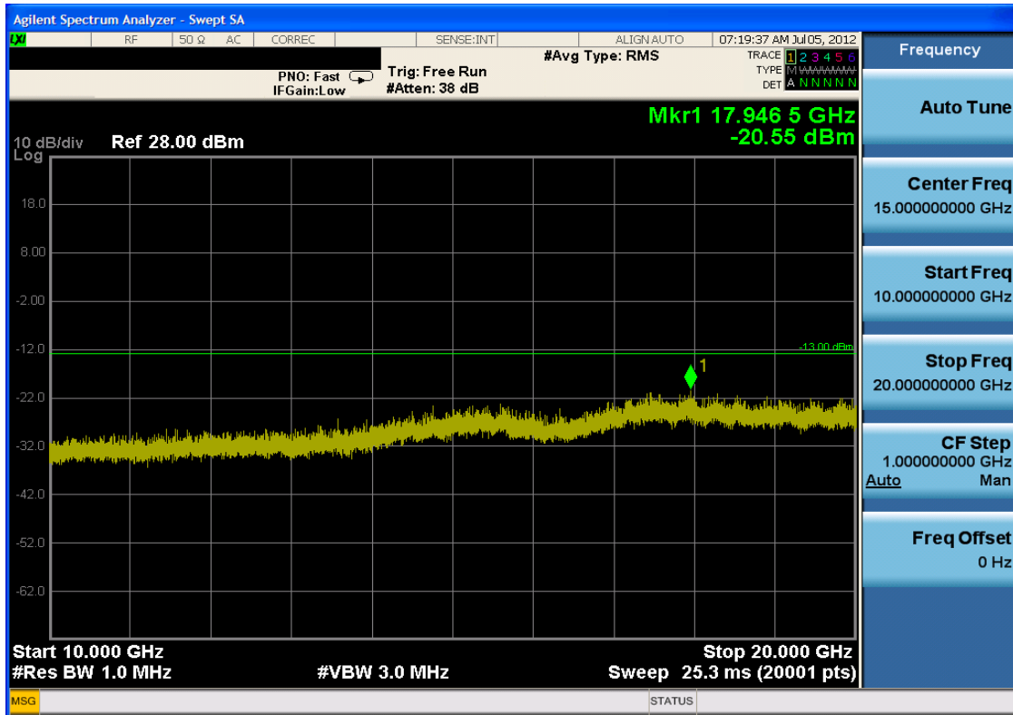
Plot 7-10. Conducted Spurious Plot (PCS CDMA Mode – Ch. 1175)
