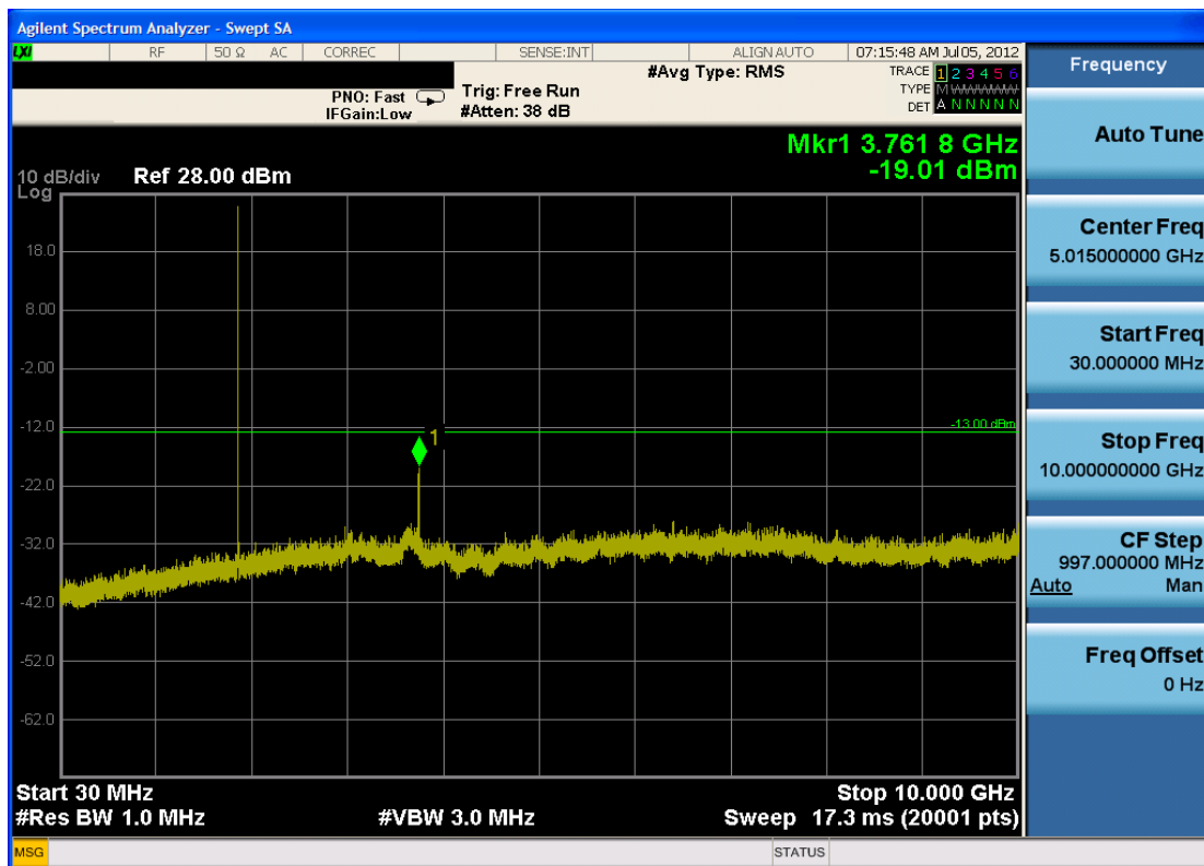
Plot 7-5. Conducted Spurious Plot (PCS CDMA Mode – Ch. 600)
