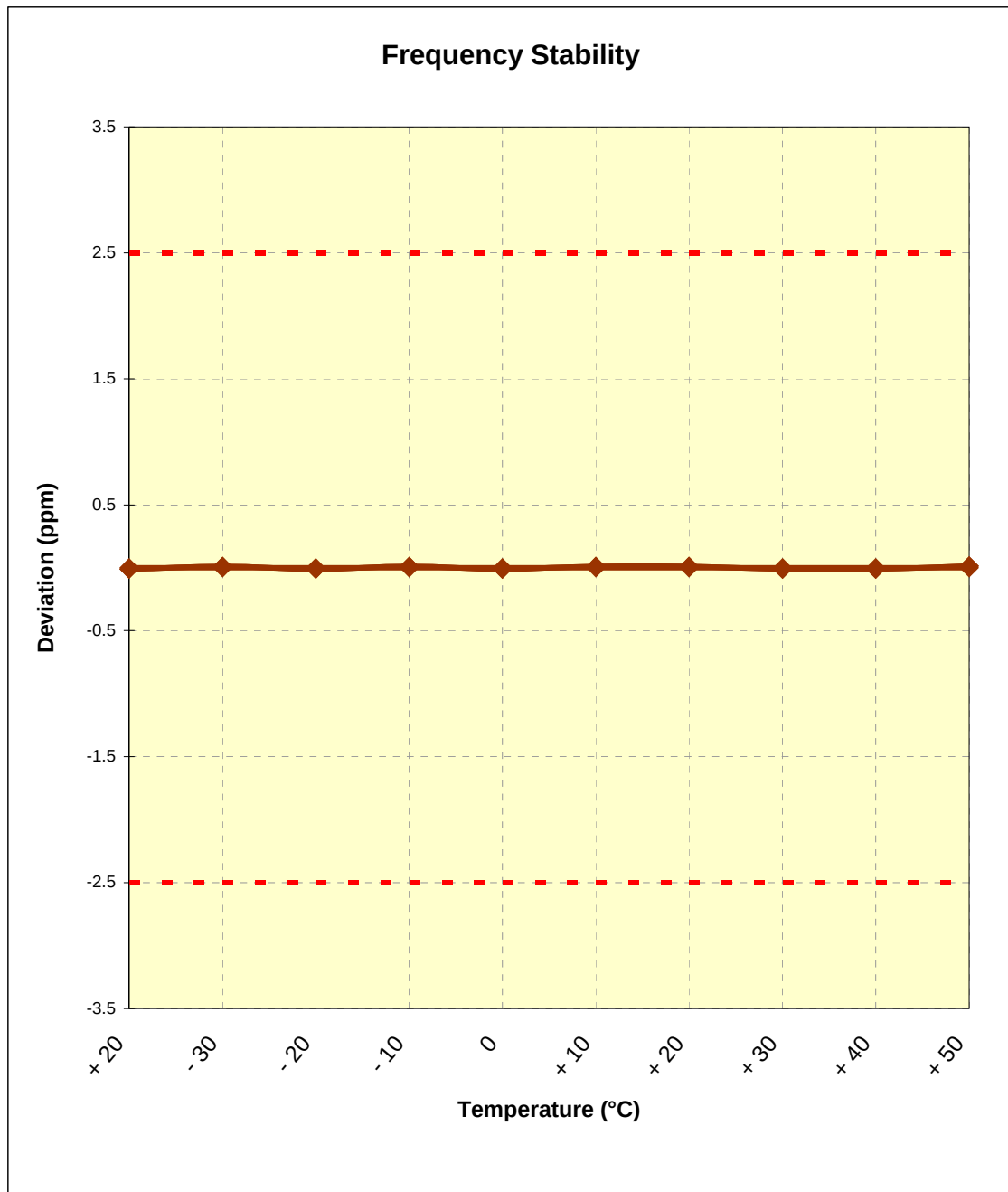
Figure 6-1. Frequency Stability Graph (PCS CDMA Mode – Ch. 600)
