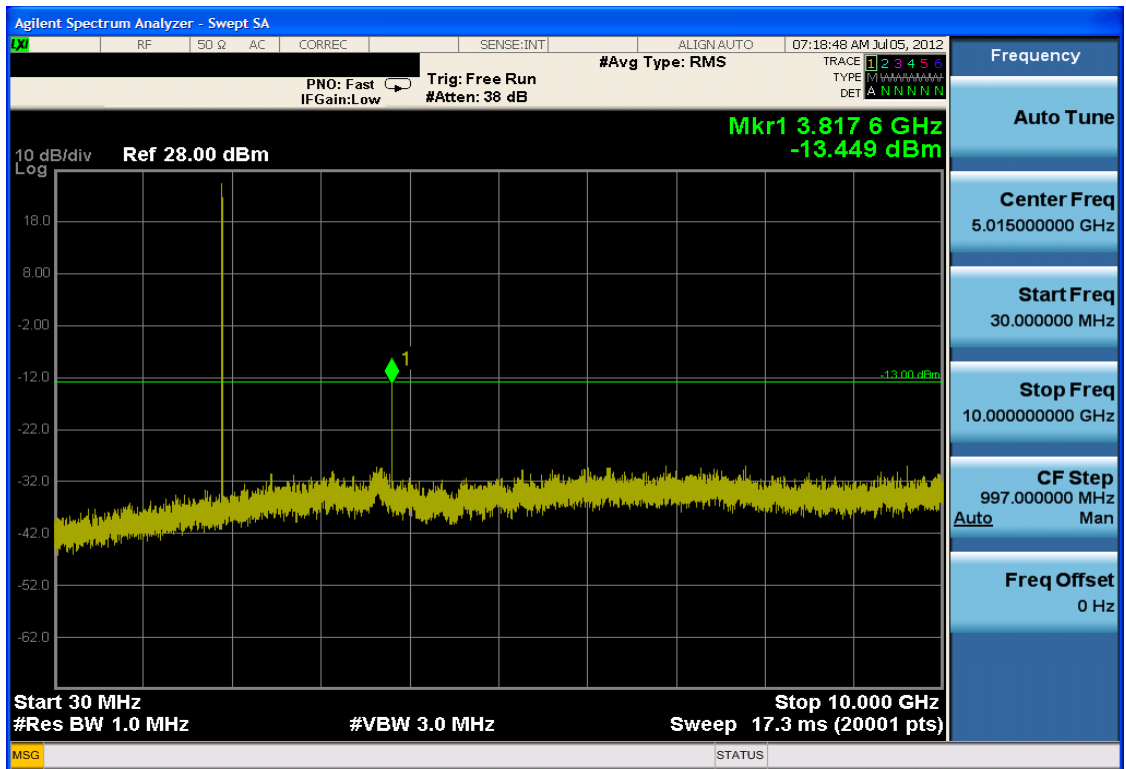
Plot 7-9. Conducted Spurious Plot (PCS CDMA Mode – Ch. 1175)
