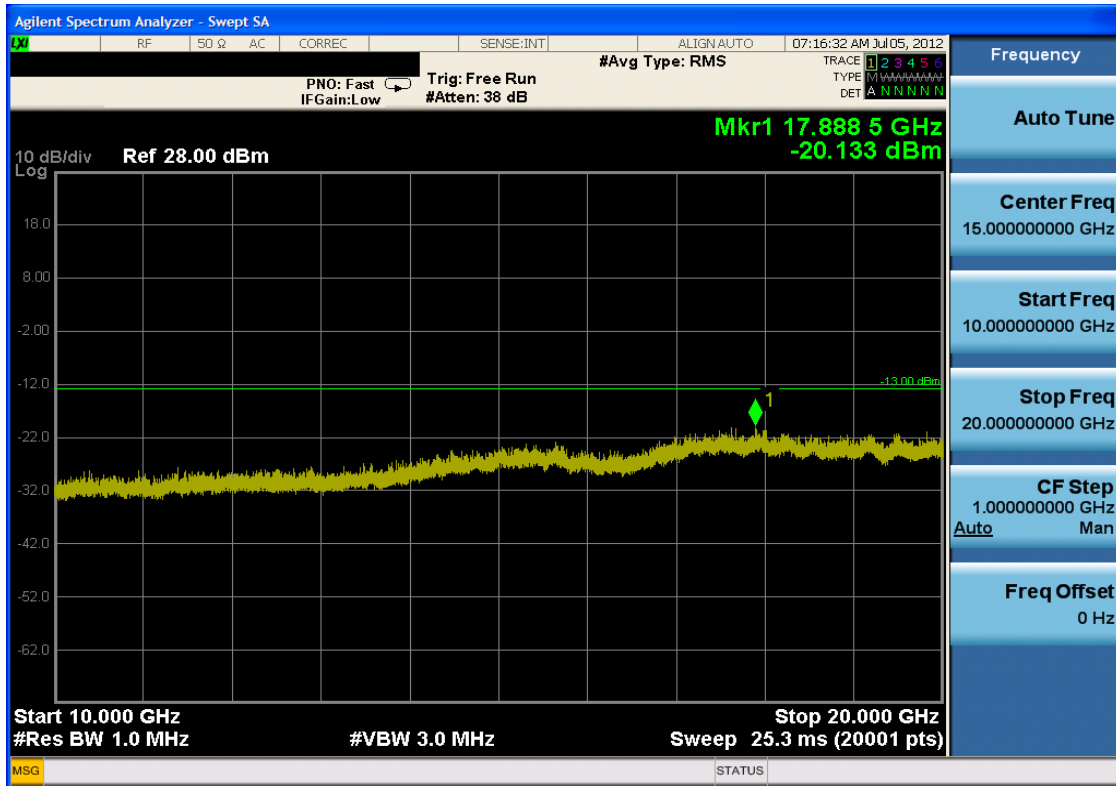
Plot 7-6. Conducted Spurious Plot (PCS CDMA Mode – Ch. 600)
