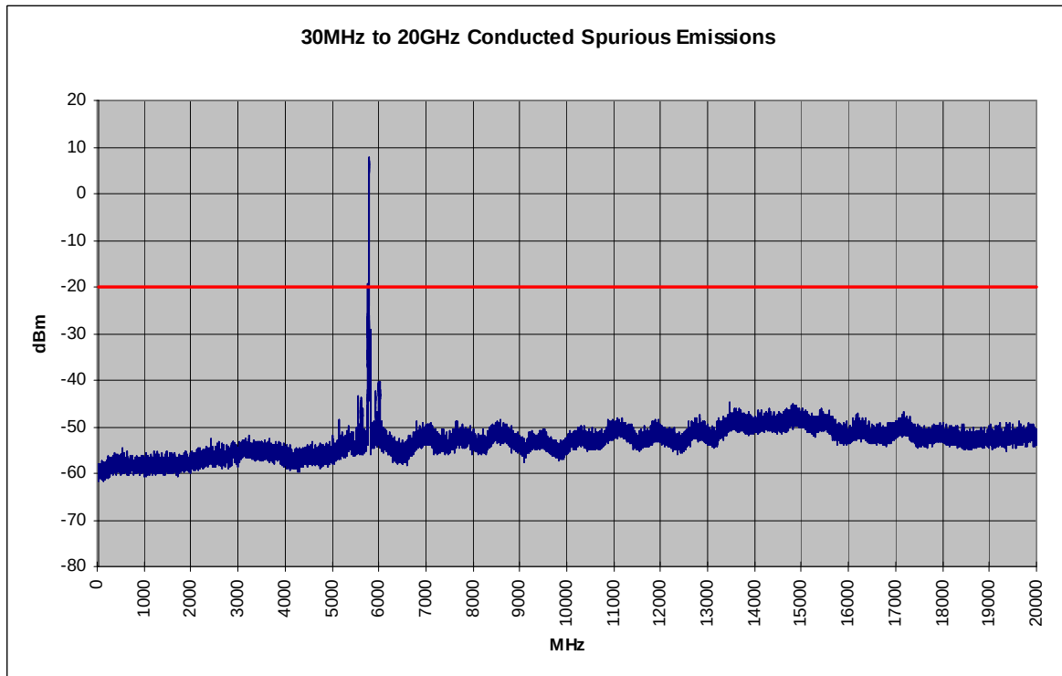
Plot 6-49. Conducted Spurious Plot (802.11a – Ch. 157)
