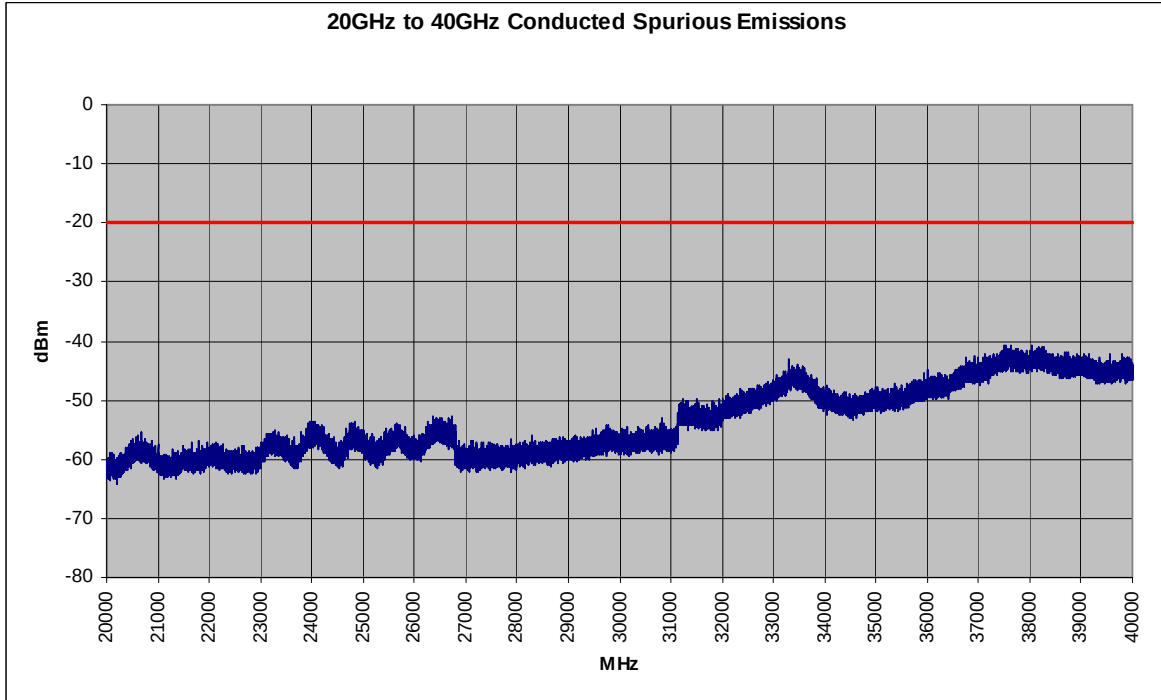
Plot 6-50. Conducted Spurious Plot (802.11a – Ch. 157)
