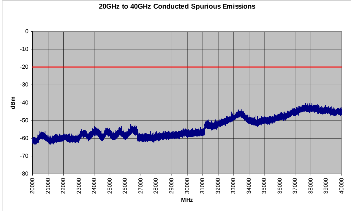
Plot 6-48. Conducted Spurious Plot (802.11a – Ch. 149)
