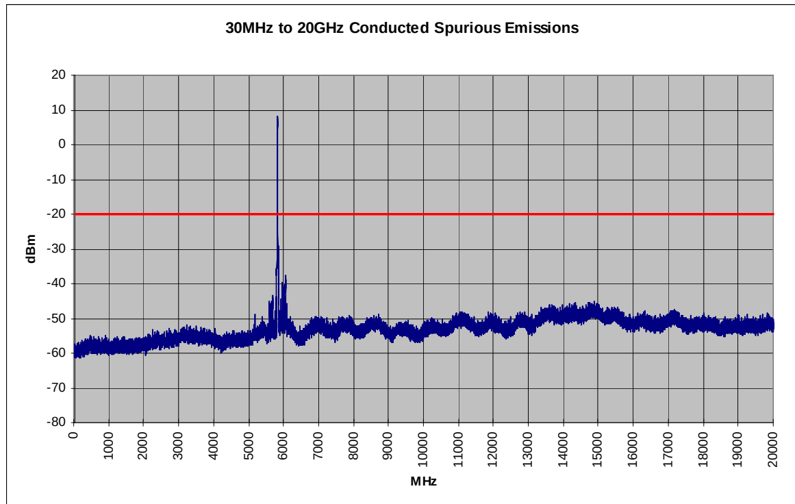
Plot 6-51. Conducted Spurious Plot (802.11a – Ch. 165)
