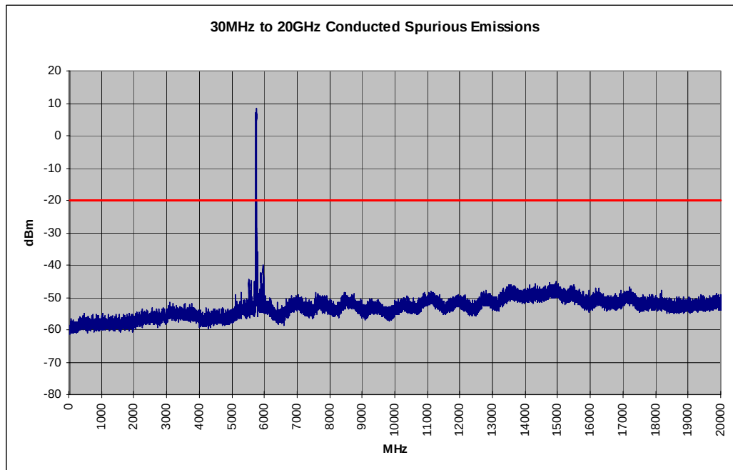
Plot 6-47. Conducted Spurious Plot (802.11a – Ch. 149)
