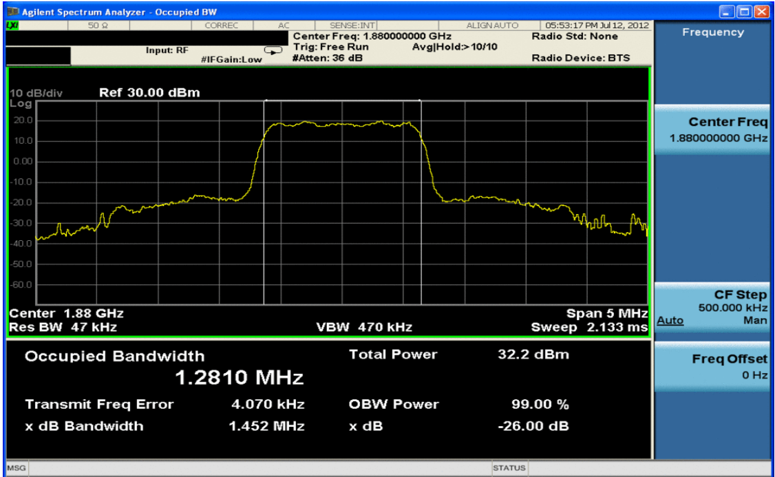
Plot 7-7. Occupied Bandwidth Plot (PCS CDMA Mode – Ch. 600)
