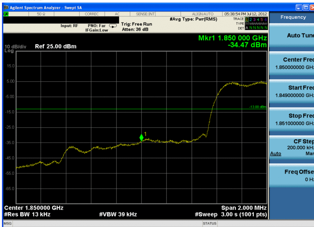
Plot 7-3. Band Edge Plot (PCS CDMA Mode – Ch. 25)
