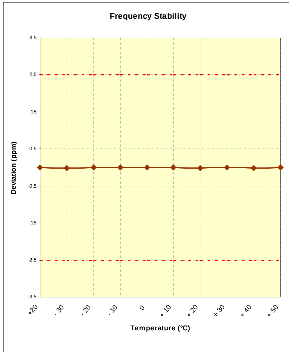
Figure 6-1. Frequency Stability Graph (PCS CDMA Mode – Ch. 600)
