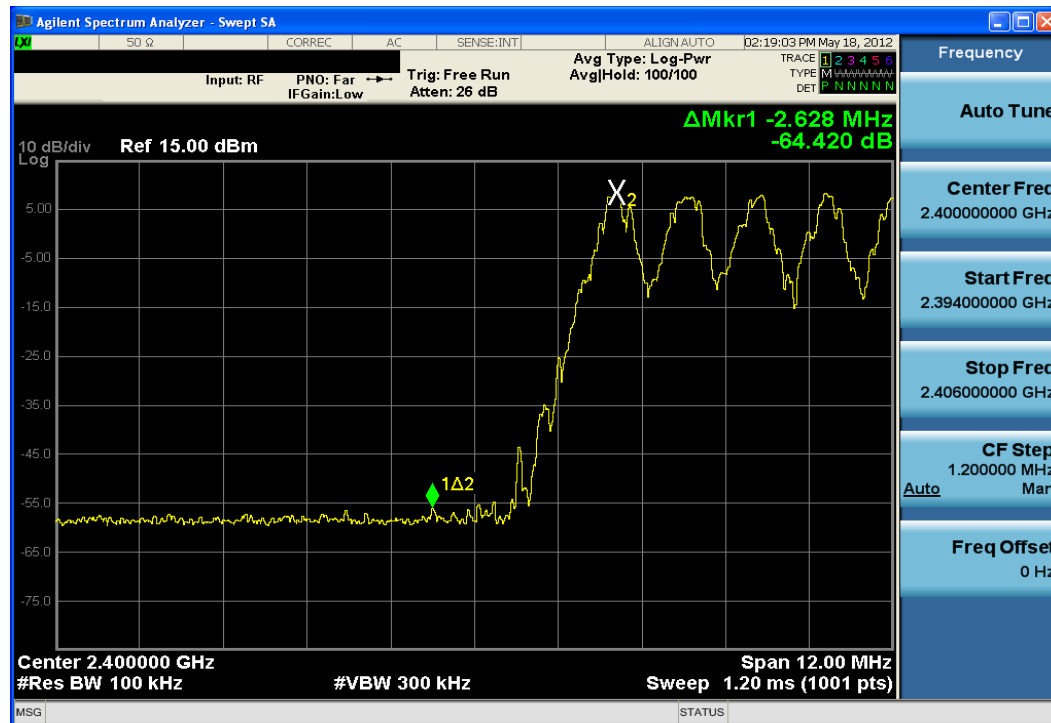
Plot 6-12. Band Edge Plot (Bluetooth with Hopping Enabled, 1Mbps)
