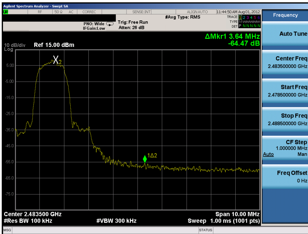
Plot 6-11. Band Edge Plot (Bluetooth with Hopping Disabled, 3Mbps – Ch. 78)
