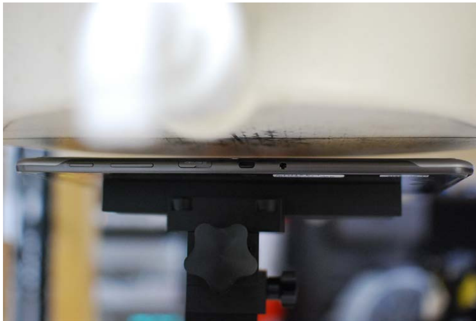
SAR Test Setup Photo 2 – Back Side at 1.1 cm
