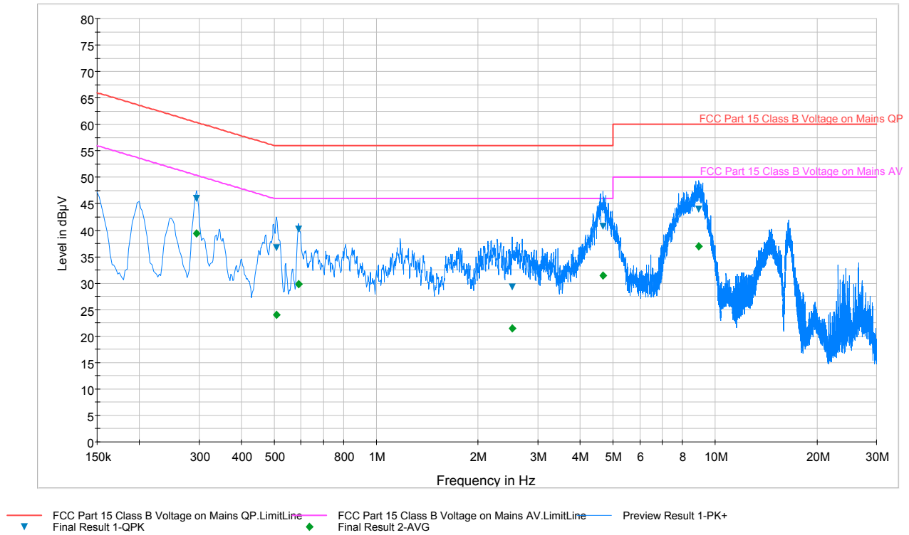
Plot 6-42. Line-Conducted Test Plot (L1)
