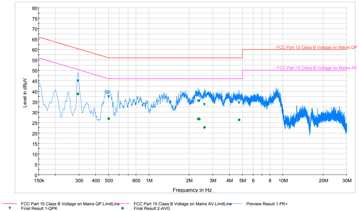
Plot 6-43. Line-Conducted Test Plot (N)
