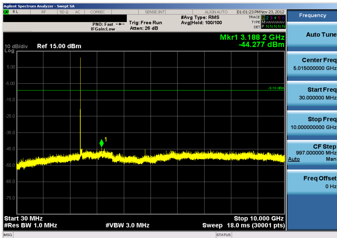
Plot 6-36. Conducted Spurious Plot (Bluetooth, 1Mbps – Ch. 0)
