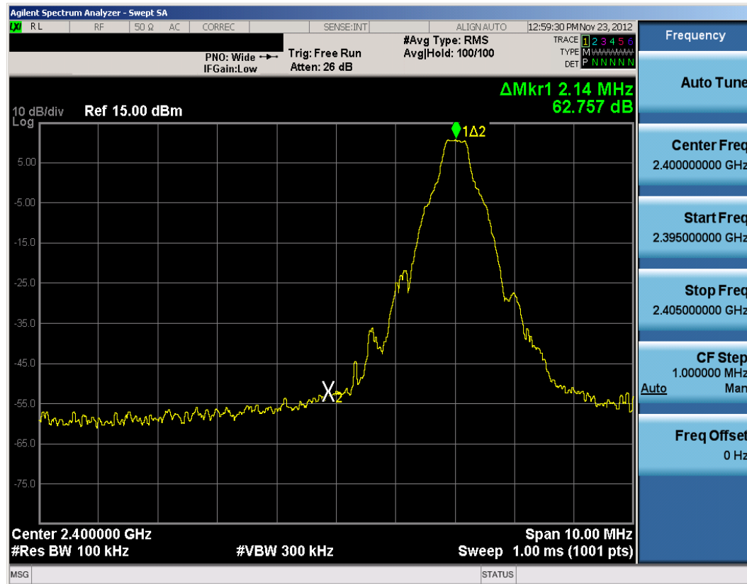
Plot 6-28. Band Edge Plot (Bluetooth with Hopping Disabled, 1Mbps – Ch. 0)
