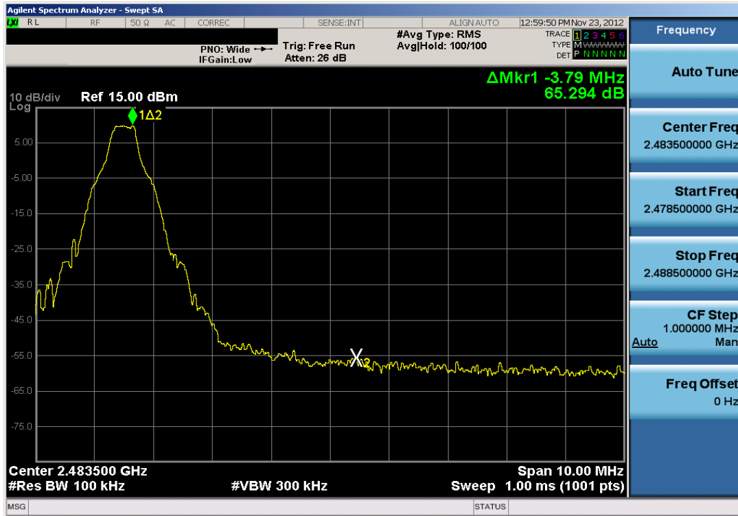
Plot 6-29. Band Edge Plot (Bluetooth with Hopping Disabled, 1Mbps – Ch. 78)
