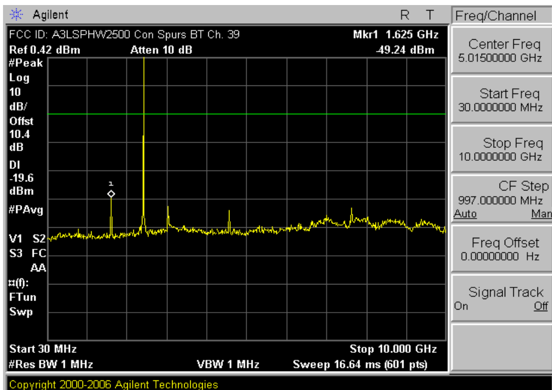
Plot 6-14. Conducted Spurious Plot (Bluetooth – Ch. 39)
