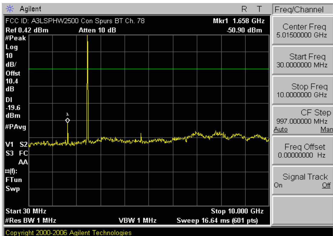
Plot 6-16. Conducted Spurious Plot (Bluetooth – Ch. 78)
