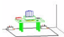
Figure 3-2. Line Conducted Emission Test Set-Up
