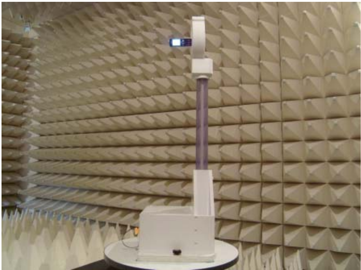
SAMSUNG FCC ID: A3LSPHW8400 1900 GSM Phone with Bluetooth.
