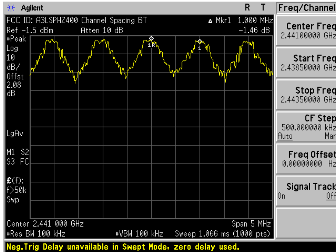
Plot 6-8. Channel Spacing Plot (Bluetooth)
