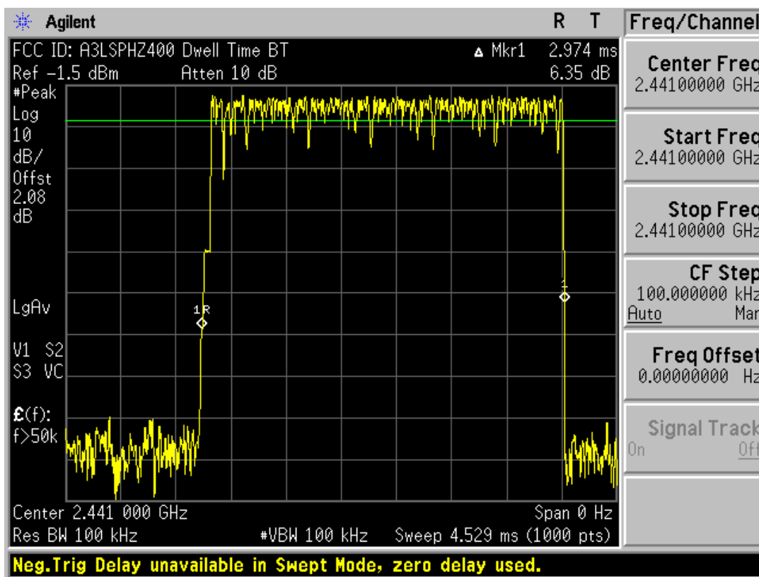
Plot 6-9. Time of Occupancy Plot (Bluetooth)
