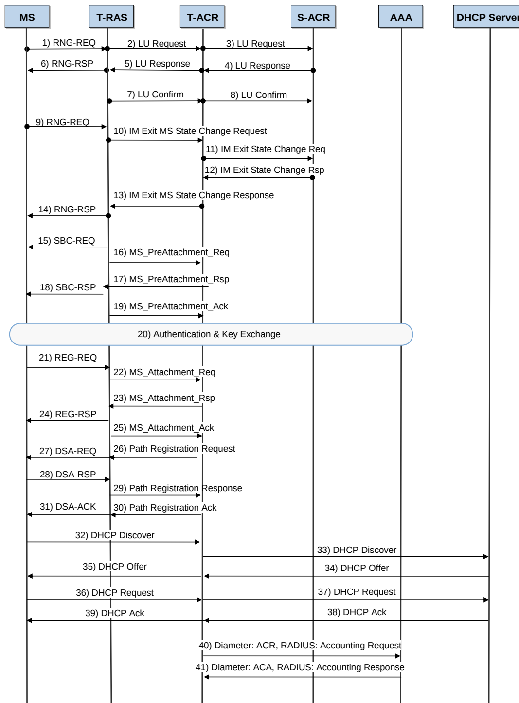
Figure 4.9 Inter-ACR Location Update Procedure (Simple IP Case)
