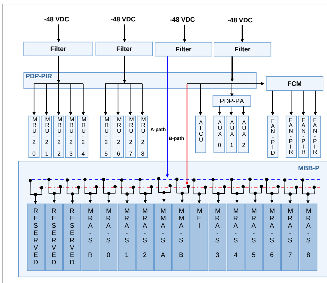
Figure 3.5 Power Structure
