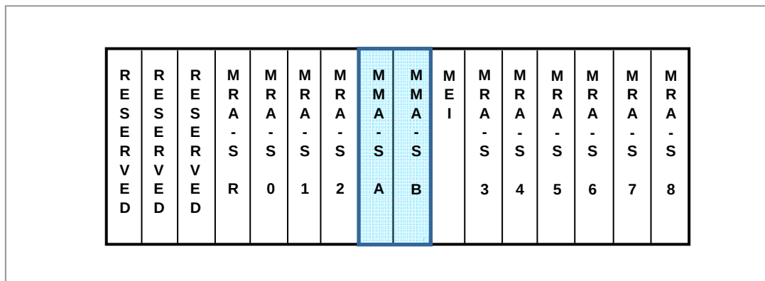
Figure 3.17 CLIM Block
