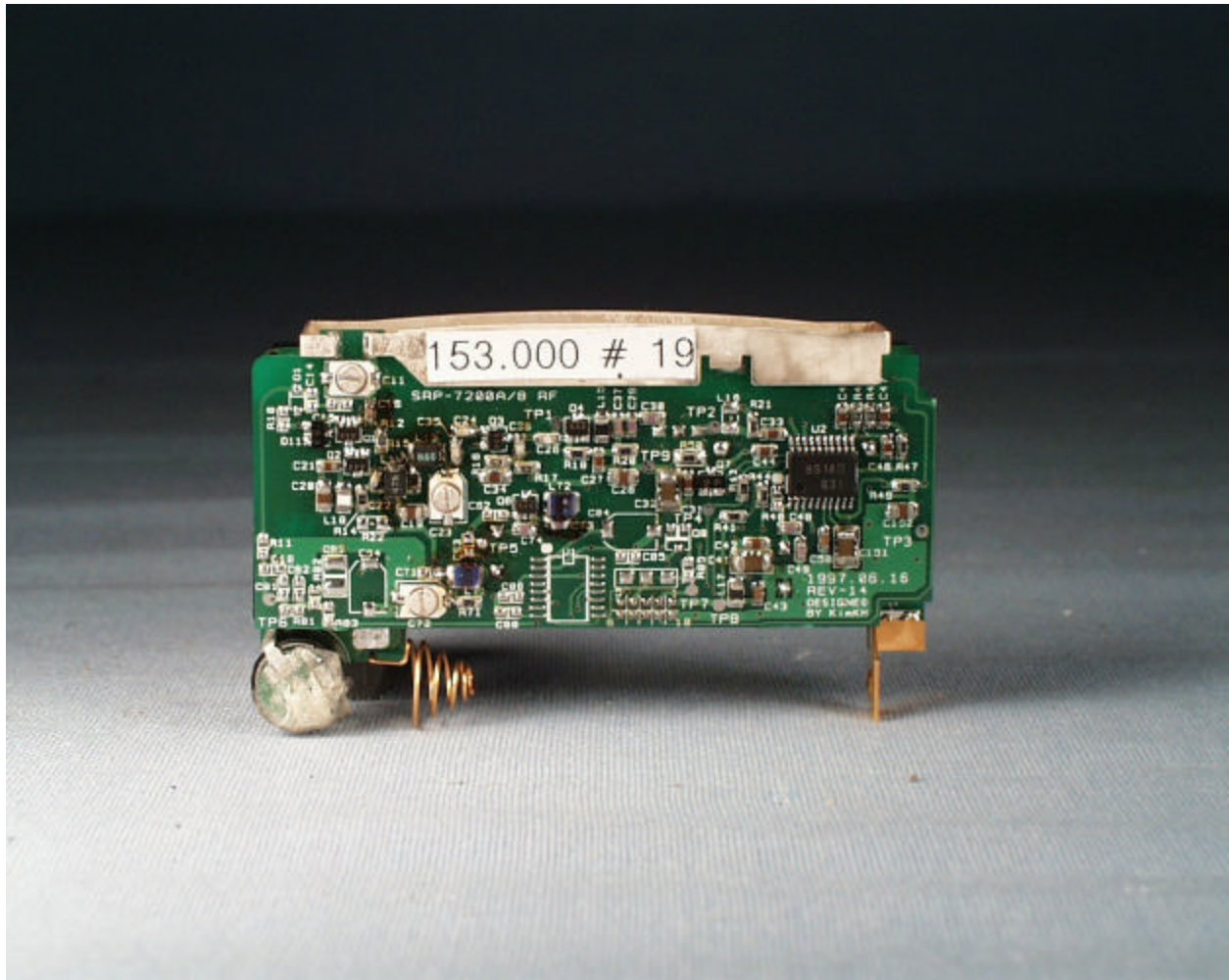
Side A (Digital Board)
