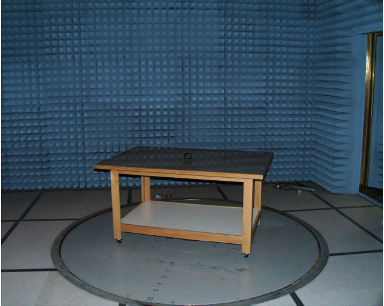
Exhibit 7: Test Set-Up Photographs
