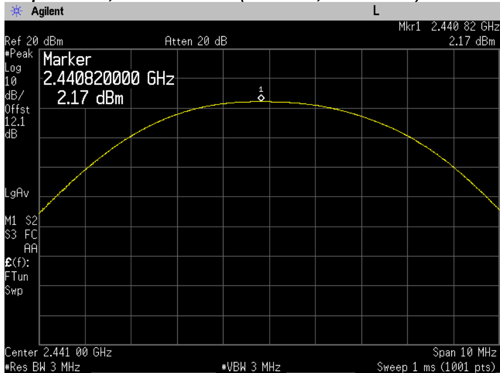
Output Power, Middle Channel (2441 MHz, GFSK Mode)
