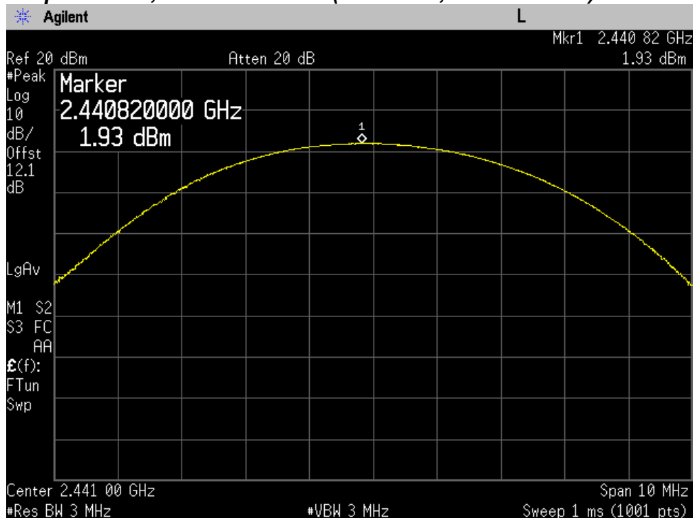
Output Power, Middle Channel (2441 MHz, 8DPSK Mode)
