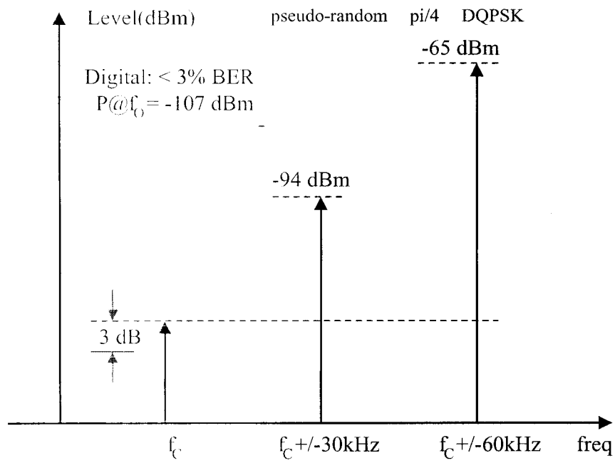
Figure 1-6. Adjacent and Alternate Channel Desensitization
