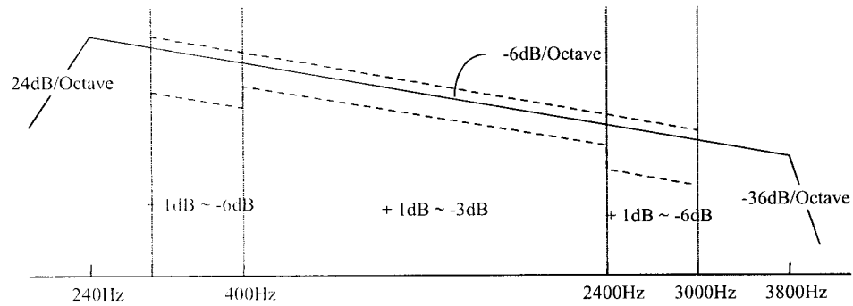
Figure1-1. Audio Frequency Output
