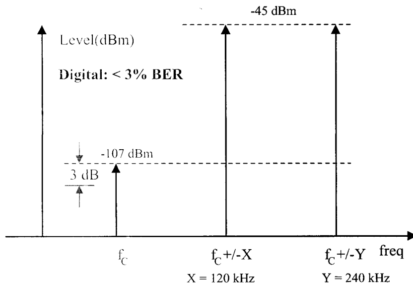
Figure 1-7. Intermodulation Spurious Response Attenuation
