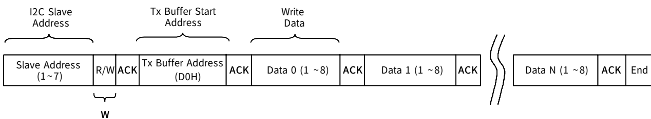
Figure 13. Tx Data Buffer Write Operation
