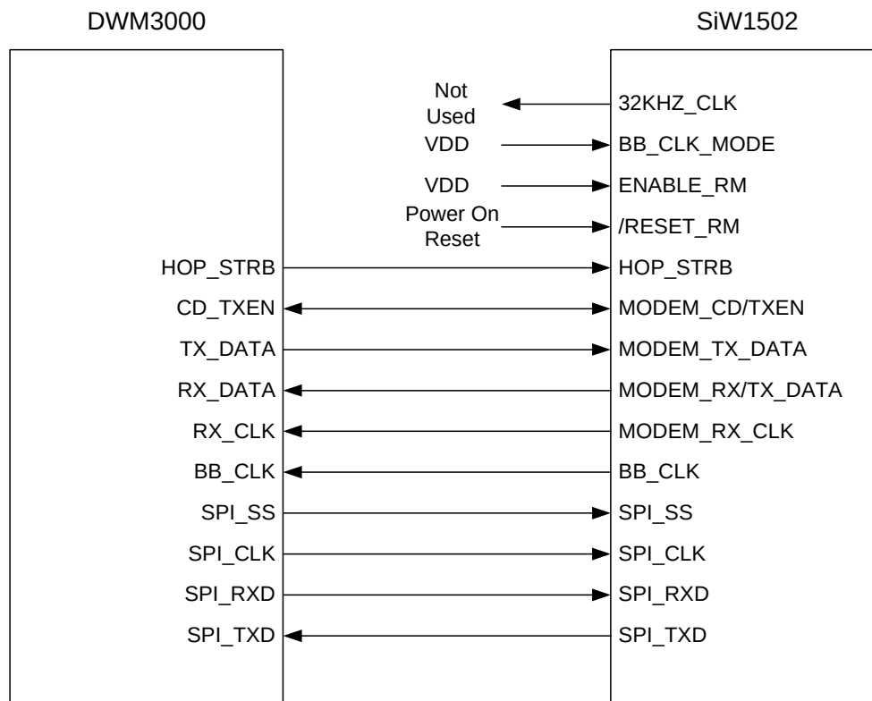
Figure 4. Connection between DWM3000 and SiW1502
