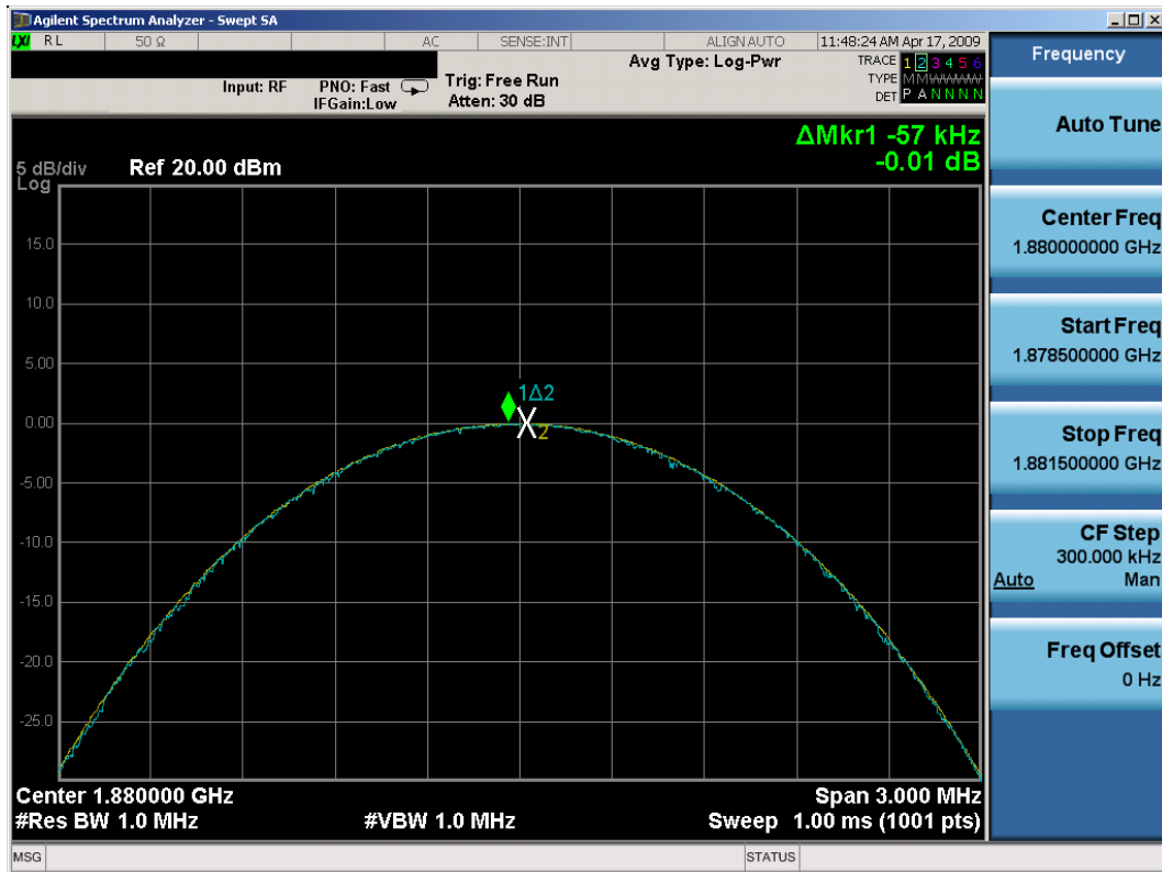
Plot 7-12. Peak-Average Ratio Plot (PCS EDGE Mode – Ch. 661)
