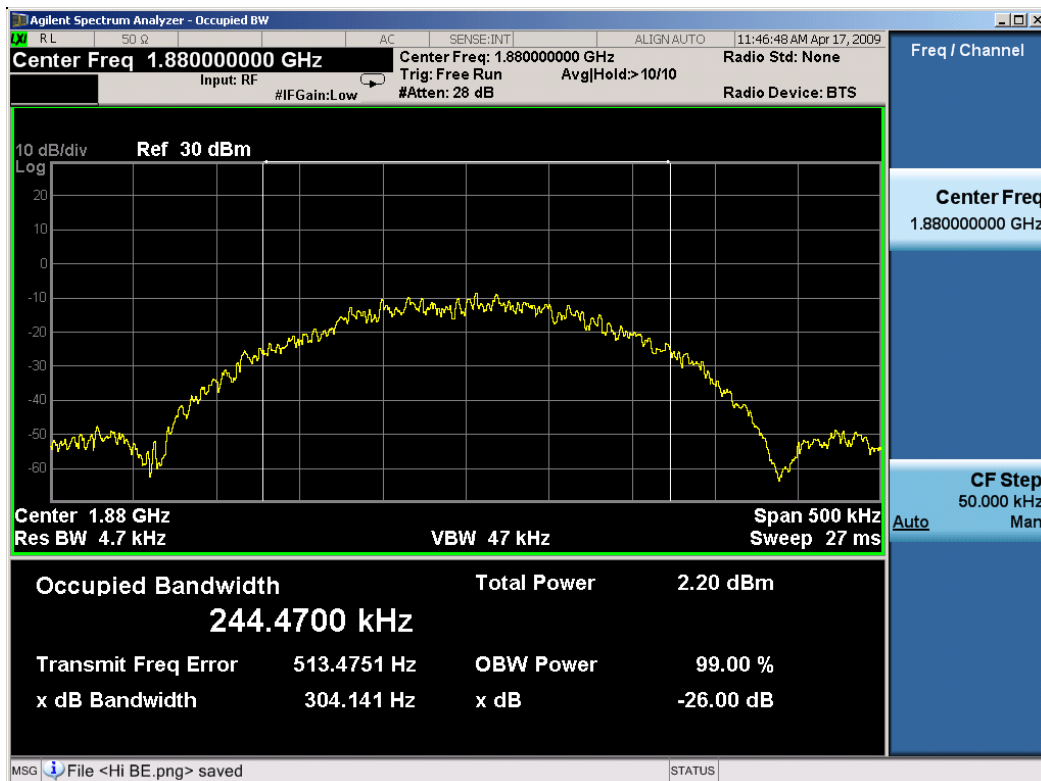
Plot 7-10. Occupied Bandwidth Plot (EDGE1900 Mode – Ch. 661)
