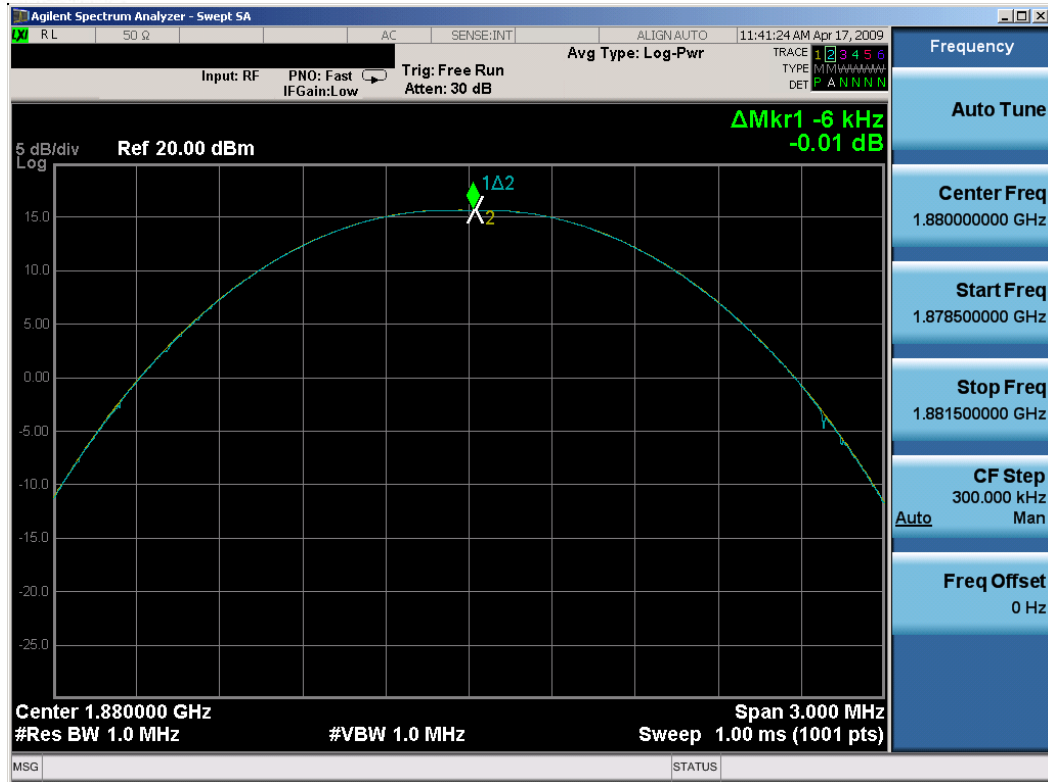
Plot 7-11. Peak-Average Ratio Plot (PCS GSM Mode – Ch. 661)
