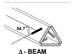
Figure 3.3 Triangular Probe Configuration
