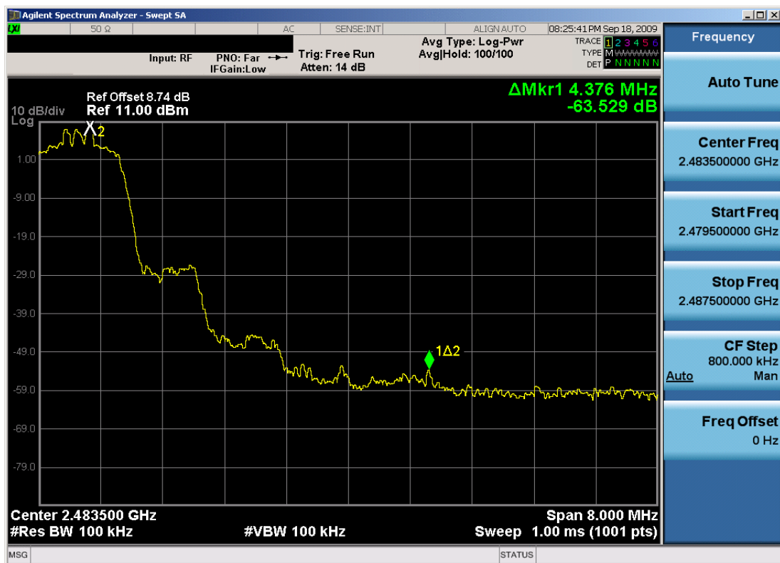
Plot 6-7. Band Edge Plot (Bluetooth 2.0 – Ch. 78)
