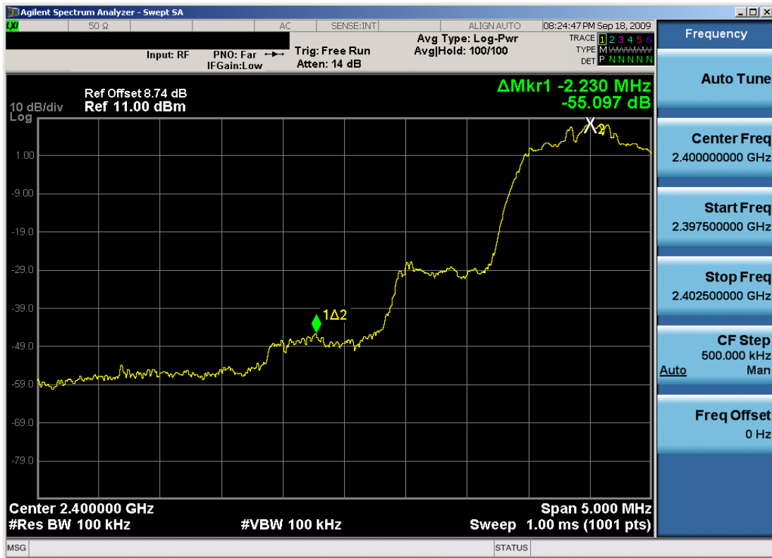
Plot 6-6. Band Edge Plot (Bluetooth 2.0 – Ch. 0)
