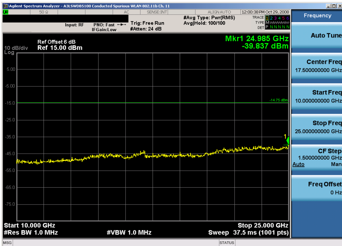
Plot 6-22. Conducted Spurious Plot (802.11b – Ch. 11)
