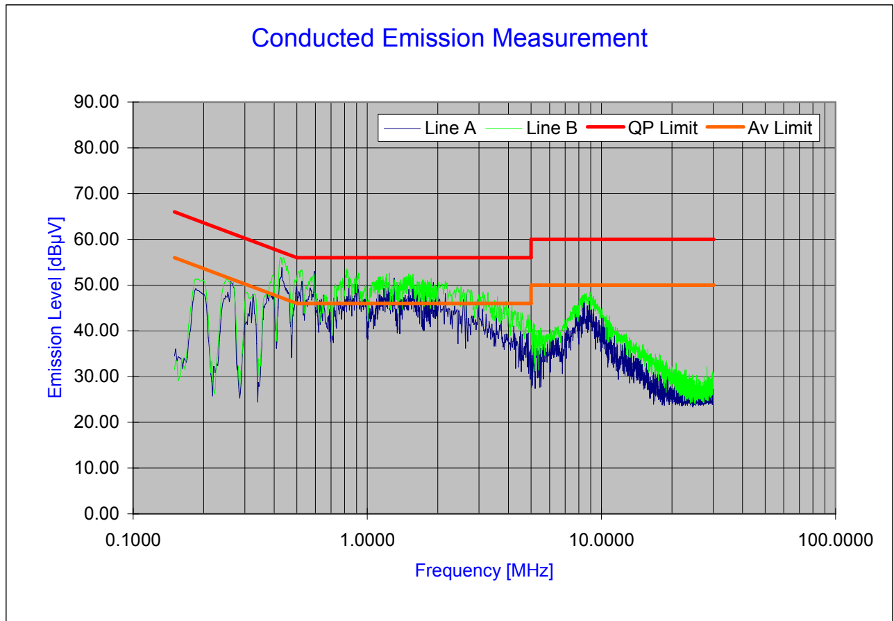
Plot 6-23. Line Conducted Plot with 802.11b
