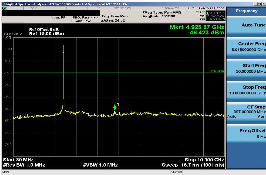
Plot 6-17. Conducted Spurious Plot (802.11b – Ch. 1)
