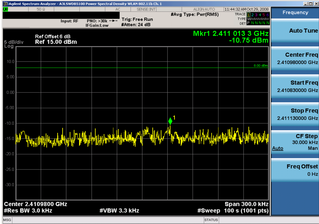
Plot 6-7. Power Spectral Density Plot (802.11b – Ch. 1)
