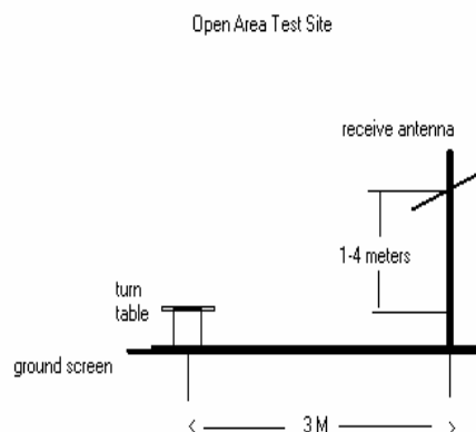
Figure 3-1. Diagram of 3-meter outdoor test range
