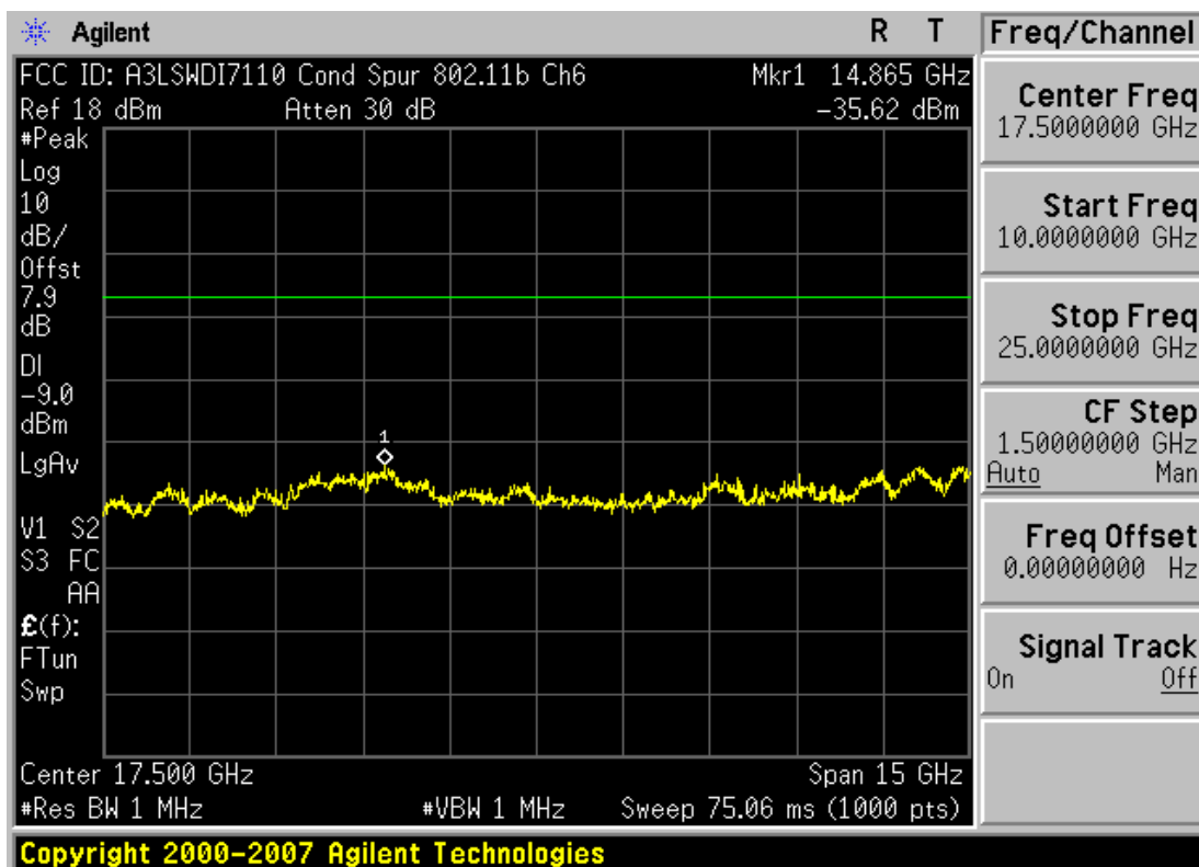
Plot 6-20. Conducted Spurious Plot (802.11b – Ch. 6)
