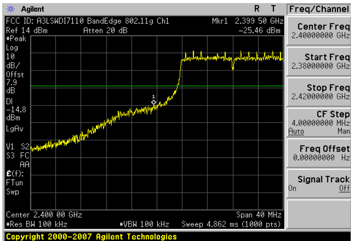
Plot 6-15. Band Edge Plot (802.11g- Ch. 1)
