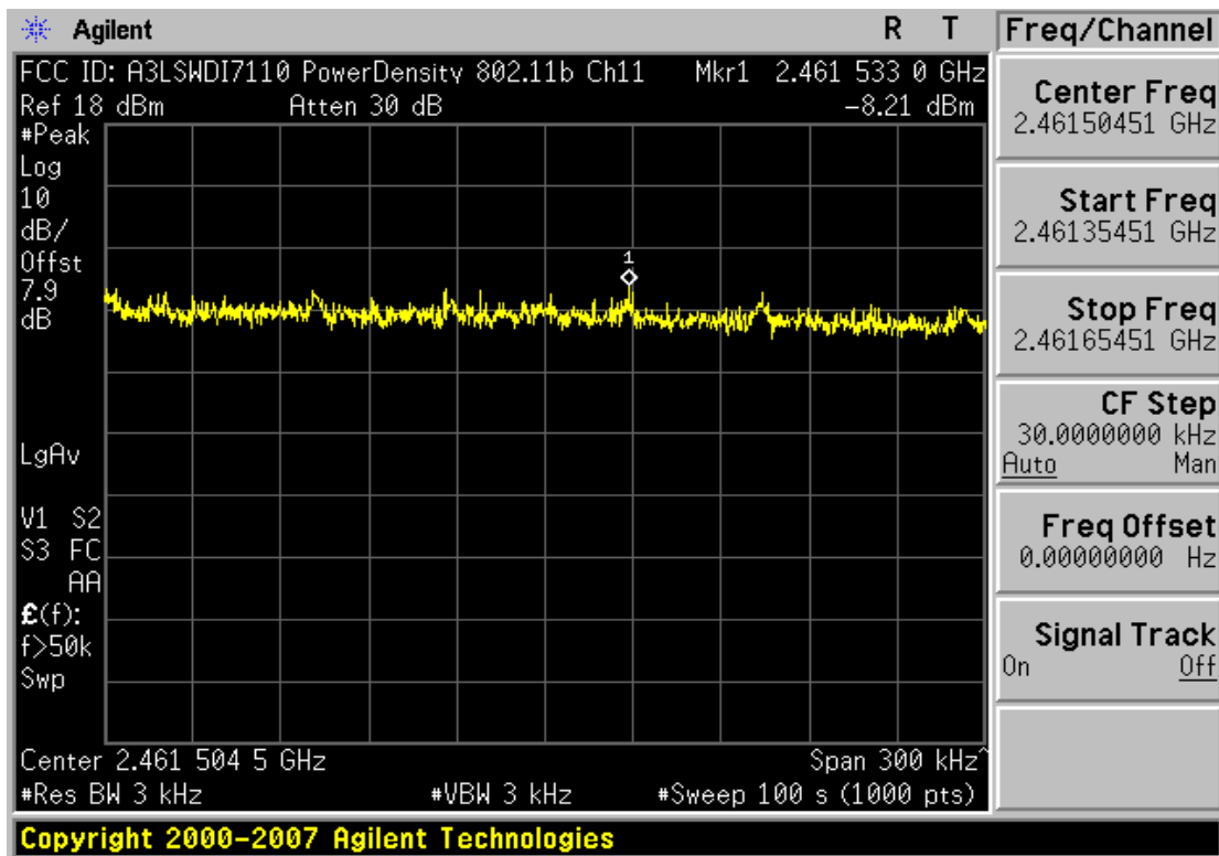
Plot 6-9. Power Spectral Density Plot (802.11b – Ch. 11)
