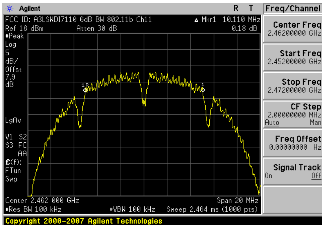
Plot 6-3. 6dB Bandwidth Plot (802.11b – Ch. 11)
