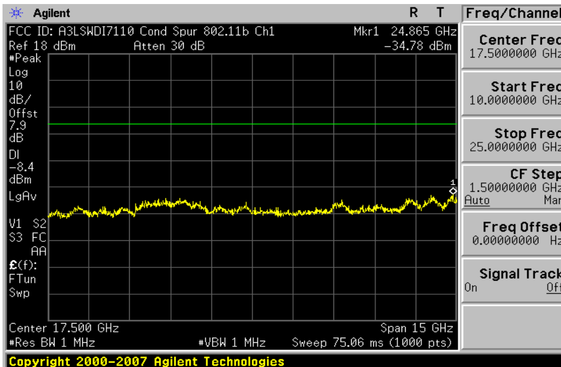
Plot 6-18. Conducted Spurious Plot (802.11b – Ch. 1)
