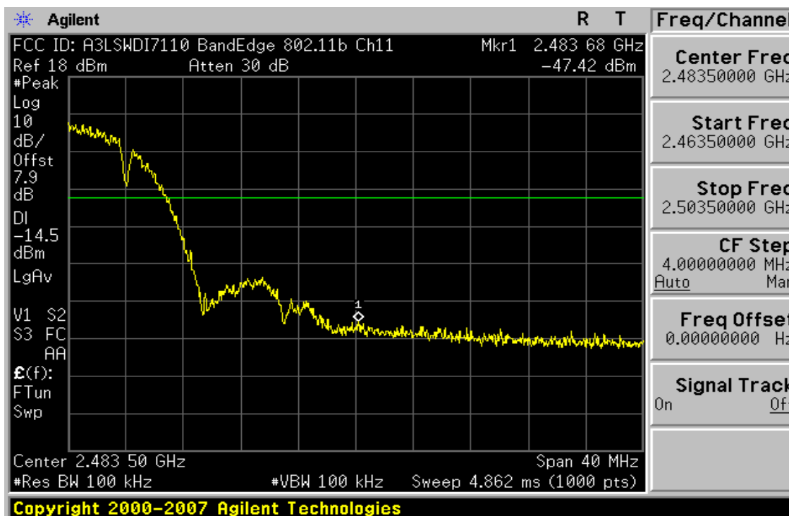
Plot 6-14. Band Edge Plot (802.11b – Ch. 11)
