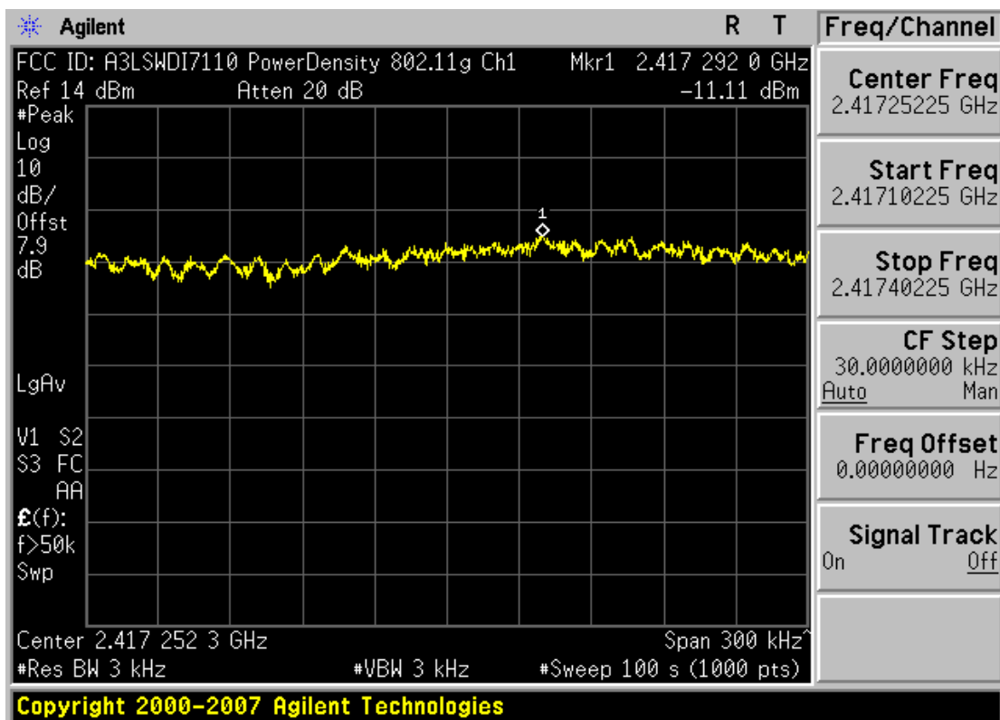
Plot 6-10. Power Spectral Density Plot (802.11g – Ch. 1)
