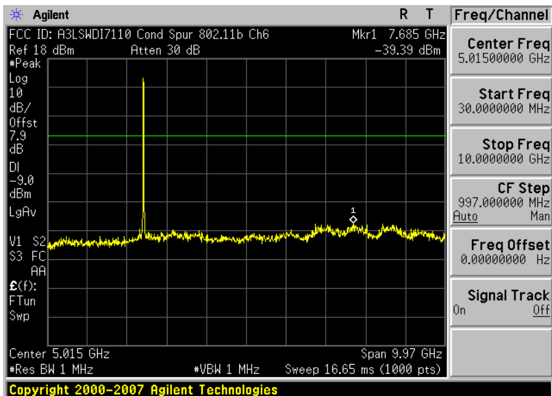
Plot 6-19. Conducted Spurious Plot (802.11b – Ch. 6)
