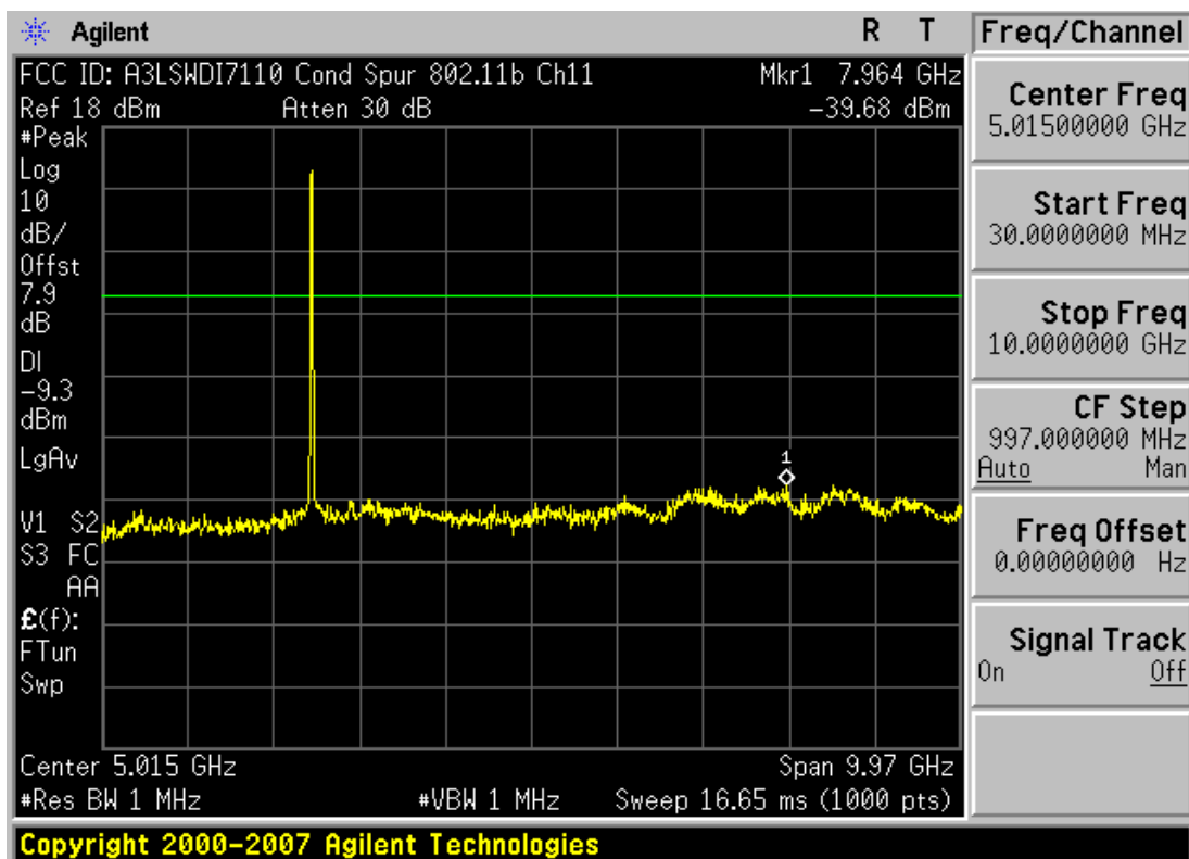
Plot 6-21. Conducted Spurious Plot (802.11b – Ch. 11)
