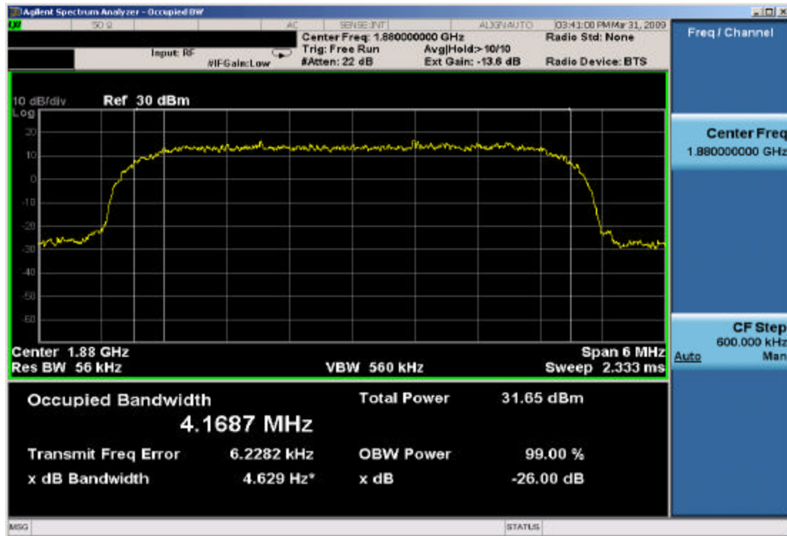
Plot 7-29. Occupied Bandwidth Plot (PCS WCDMA Mode – Ch. 9400)
