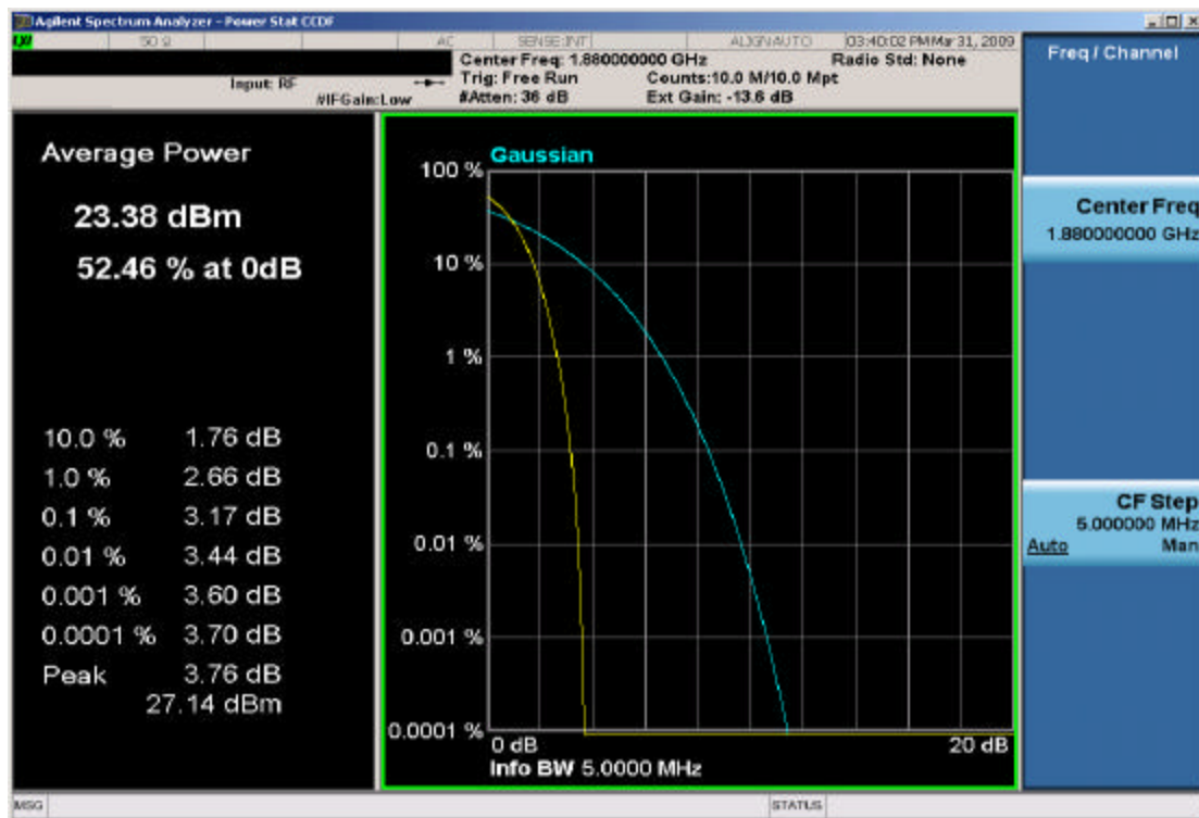
Plot 7-30. Peak-Average Ratio Plot (PCS WCDMA Mode – Ch. 9400)
