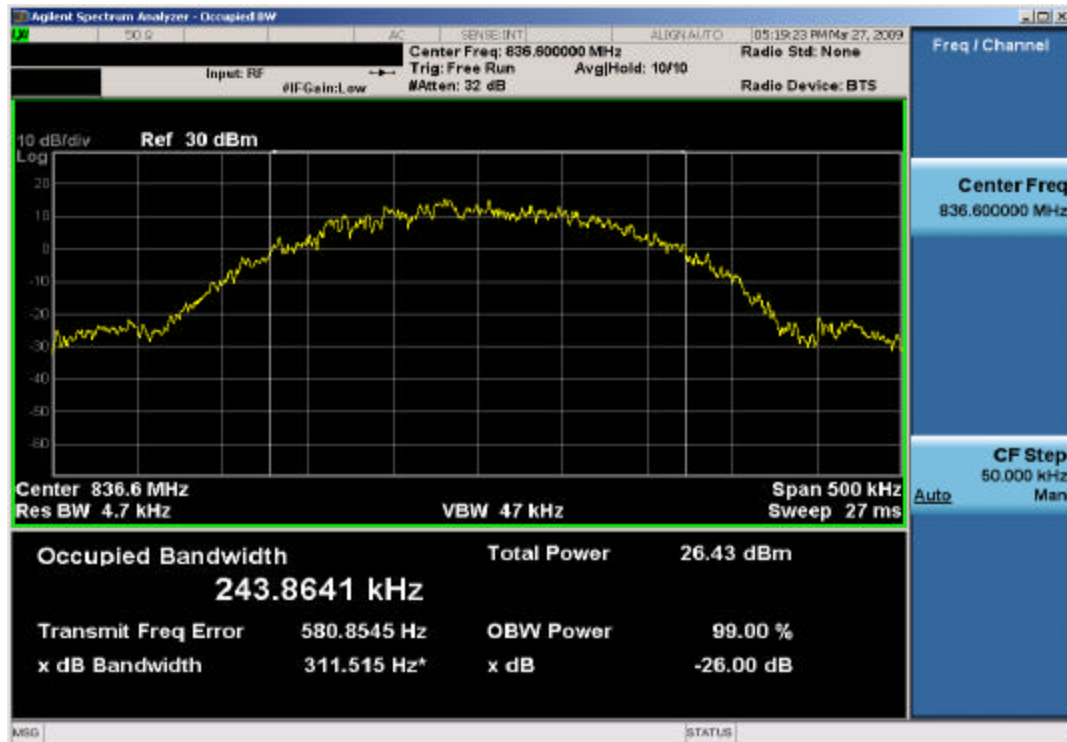
Plot 7-10. Occupied Bandwidth Plot (EDGE850 Mode – Ch. 190)
