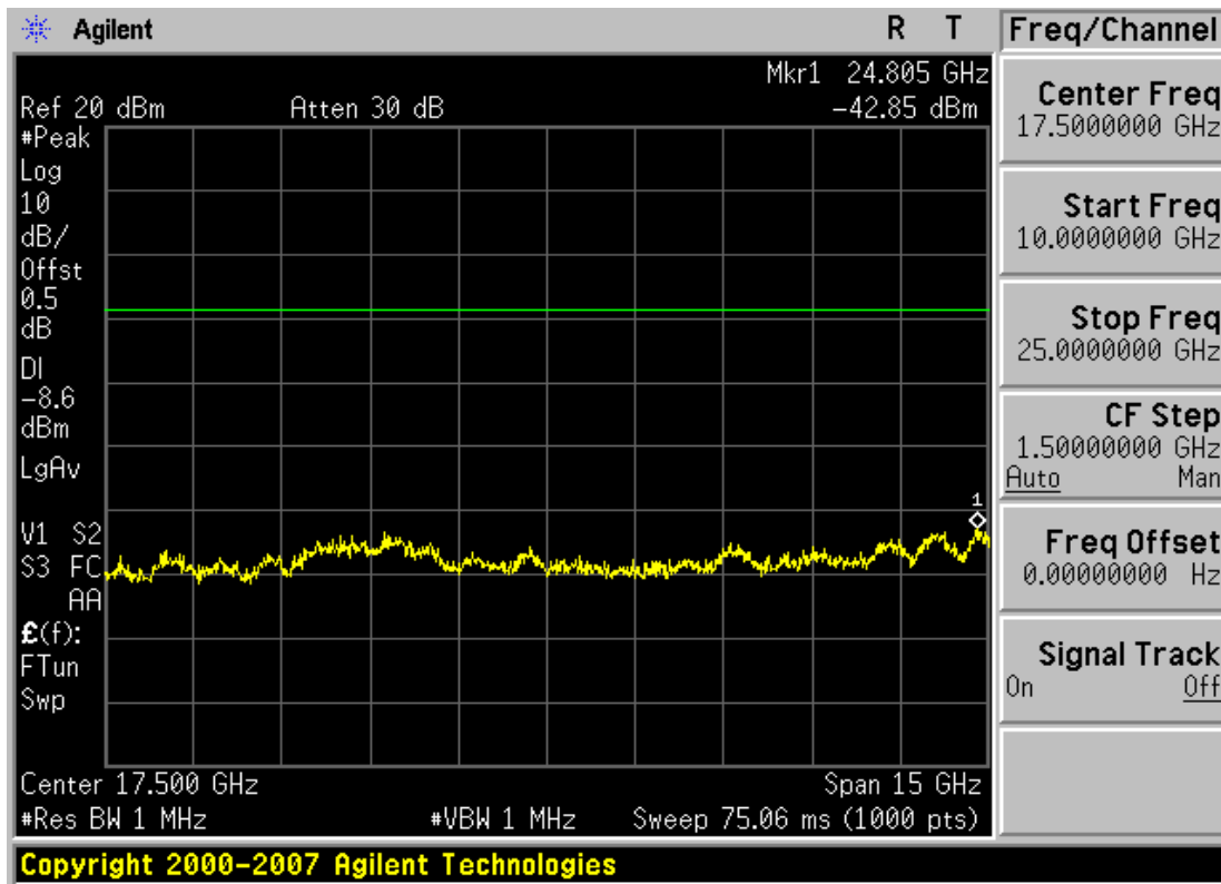
Plot 6-22. Conducted Spurious Plot (802.11b – Ch. 11)
