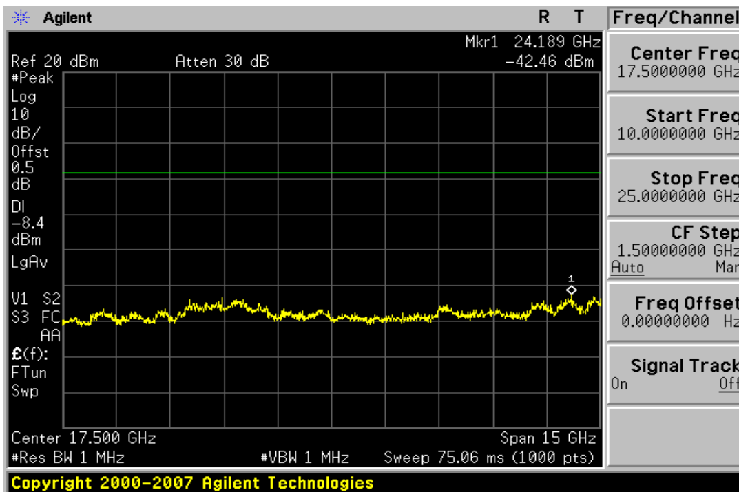
Plot 6-18. Conducted Spurious Plot (802.11b – Ch. 1)
