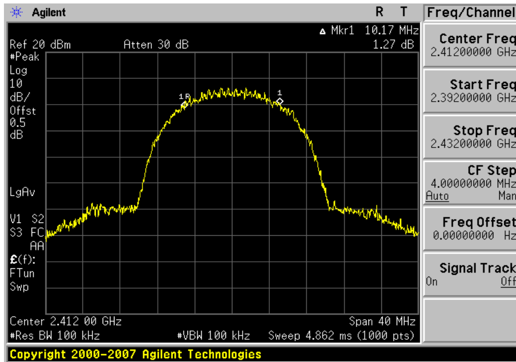
Plot 6-1. 6dB Bandwidth Plot (802.11b – Ch. 1)
