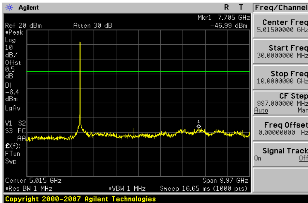
Plot 6-17. Conducted Spurious Plot (802.11b – Ch. 1)
