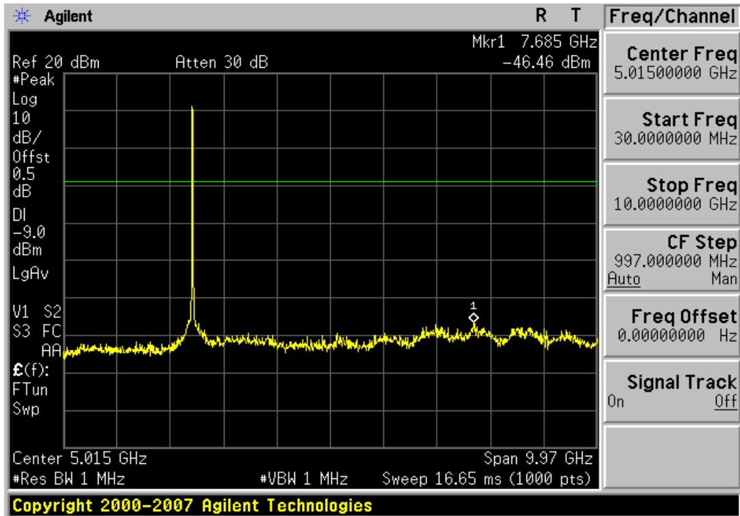
Plot 6-19. Conducted Spurious Plot (802.11b – Ch. 6)
