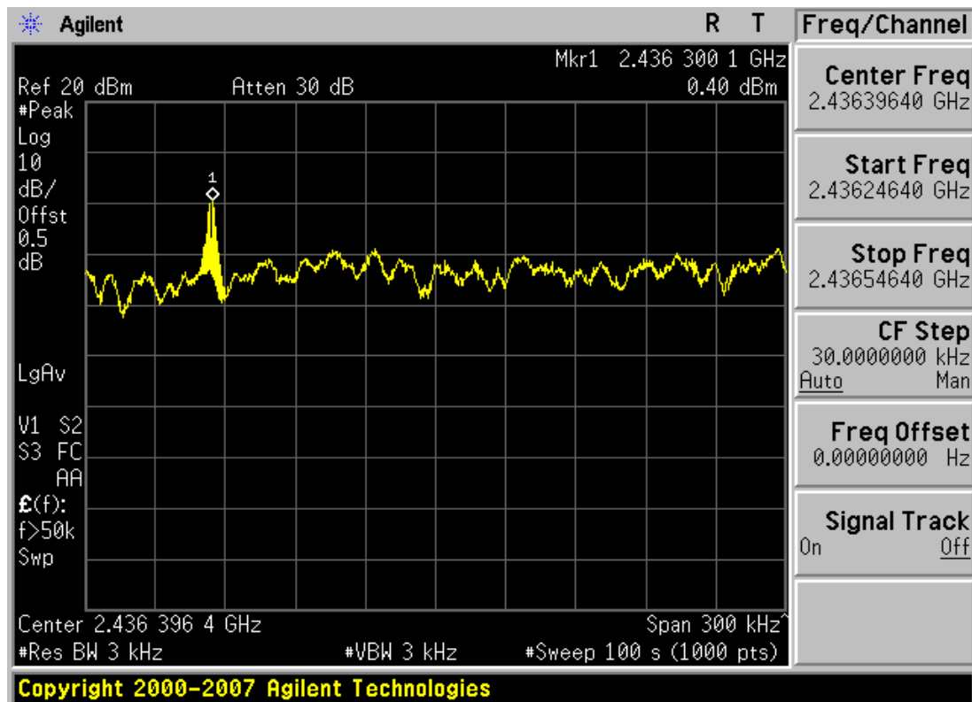
Plot 6-8. Power Spectral Density Plot (802.11b – Ch. 6)
