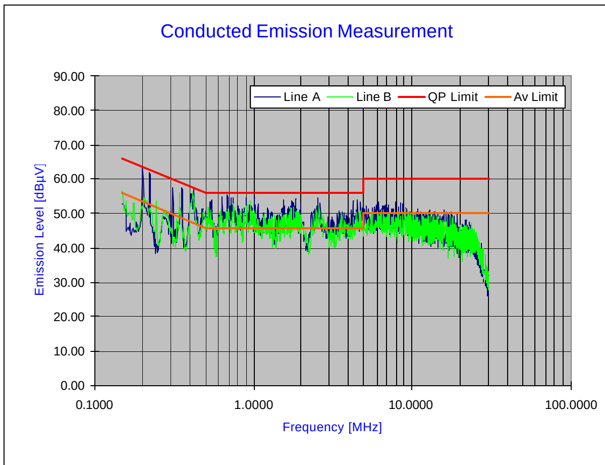
Plot 6-18. Line Conducted Plot with Bluetooth
