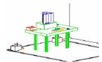
Figure 3-3. Wooden Table & Bonded LISNs
