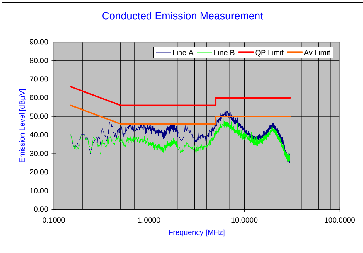
Plot 6-1. Line Conducted Plot with 802.11b
