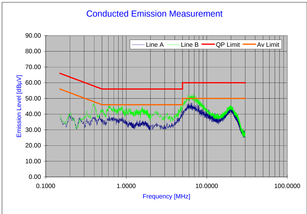
Plot 6-2. Line Conducted Plot with 802.11g
