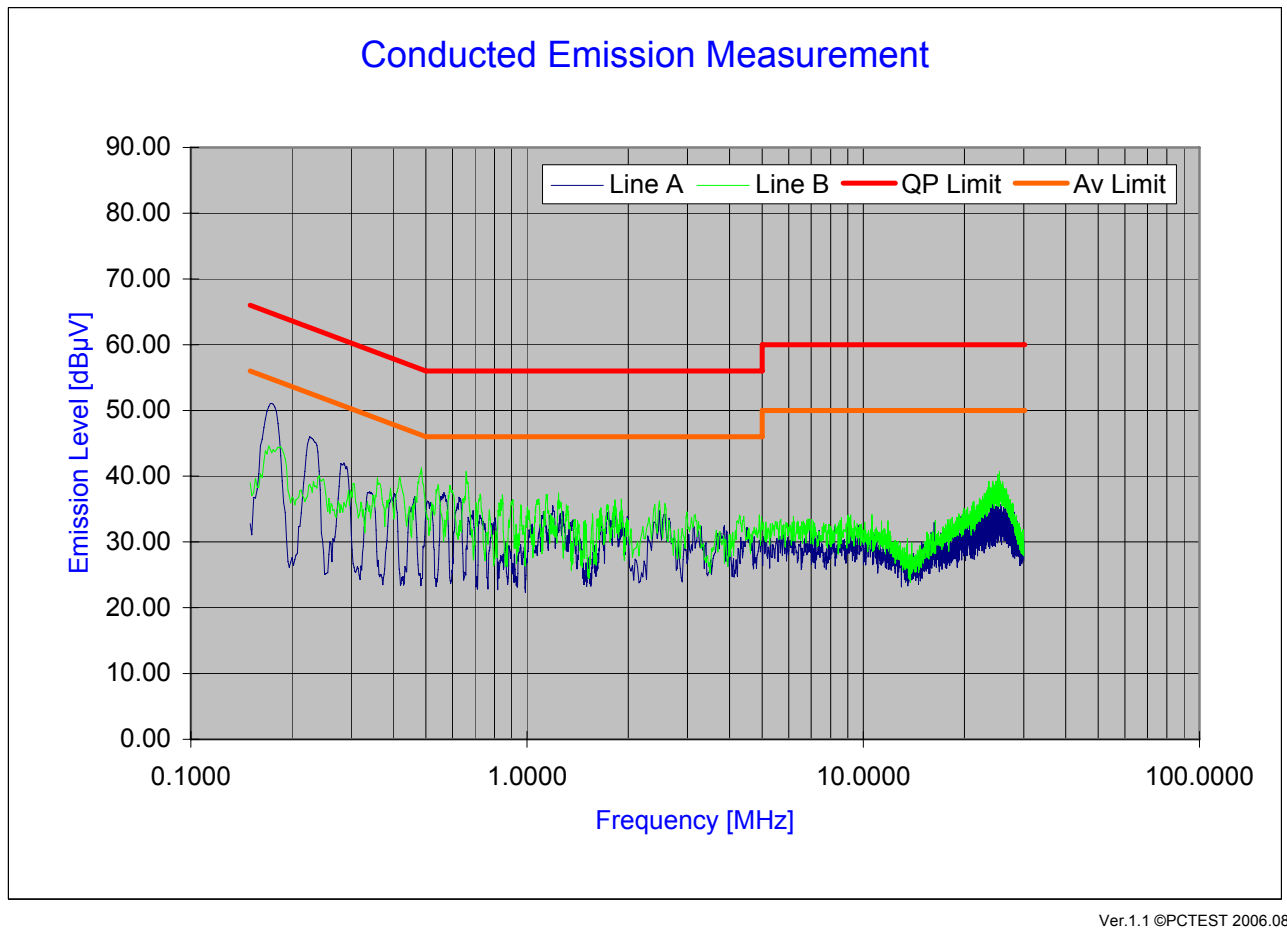
Plot 6-18. Line Conducted Plot with Bluetooth
